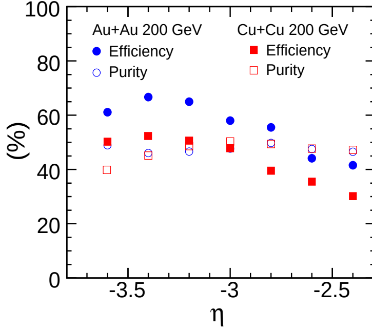
Fig. 1. (color online) Photon reconstruction efficiency ( \epsilon_\gamma ) (solid symbols) and purity of photon sample ( f_p ) (open symbols) for PMD as a function of pseudorapidity ( \eta ) for minimum bias Au+Au and Cu+Cu at \sqrt{s_{NN}} = 200 GeV.
