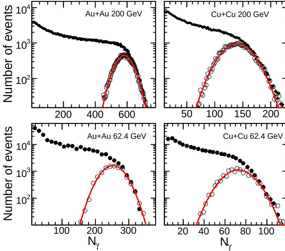
Fig. 2. (color online) Event-by-event photon multiplicity distributions (solid circles) for Au+Au and Cu+Cu at \sqrt{s_{NN}} = 62.4 and 200 GeV. The distributions for top 0–5% central Au+Au collisions and top 0–10% central Cu+Cu collisions are also shown (open circles). The photon multiplicity distributions for central collisions are observed to be Gaussian (solid line). Only statistical errors are shown.
