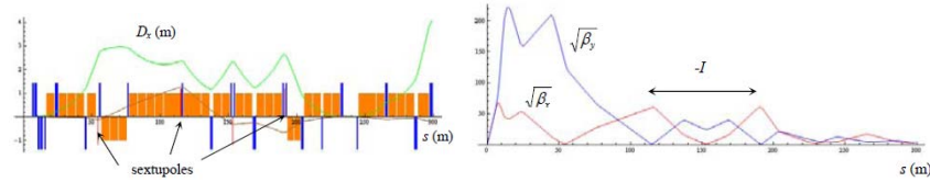
Figure 9. (left) magnet layout and dispersion function for collider interaction region; (right) interaction region beta functions.
