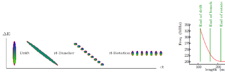
Figure 5. (left) schematic of phase rotation and bunching process; (right) frequencies of RF cavities along the channel.
