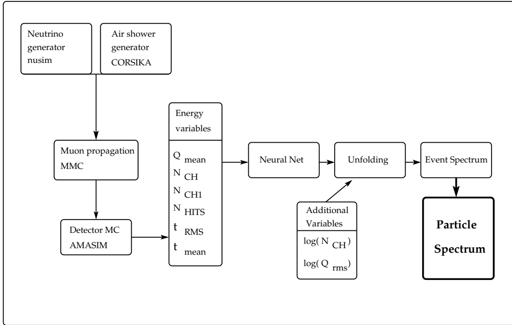
Figure 1: Scheme of the simulation and analysis chain
