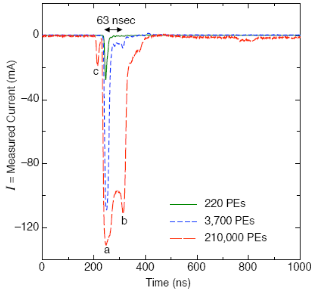
Fig.13 PMT signals for different input amplitudes, showing the effect of saturation. Saturation compresses the instantaneous current, so that small 'features' like prepulsing and afterpulsing grow in relative size when saturation sets in 56 .
