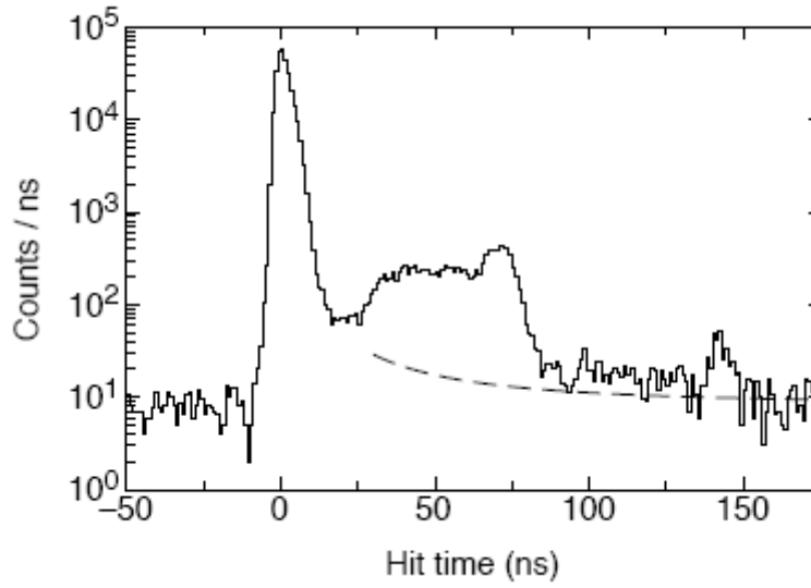
Fig.12 The distribution of arrival times of single photoelectrons at the PMT. A tail of late-arriving photons follows the main pulse 56 . The dashed line shows the contribution to late light due to laser afterglow plus random background.
