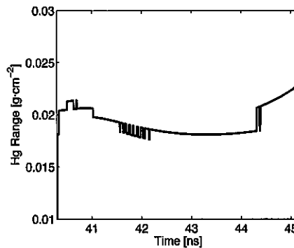
Figure 15. Range of beam ions in the 683 TW main pulse following three foot shocks ( N_s = 3 case). The mercury ions' incident kinetic energy is fixed at 2.21 GeV for the duration of the 4.2 ns pulse.
