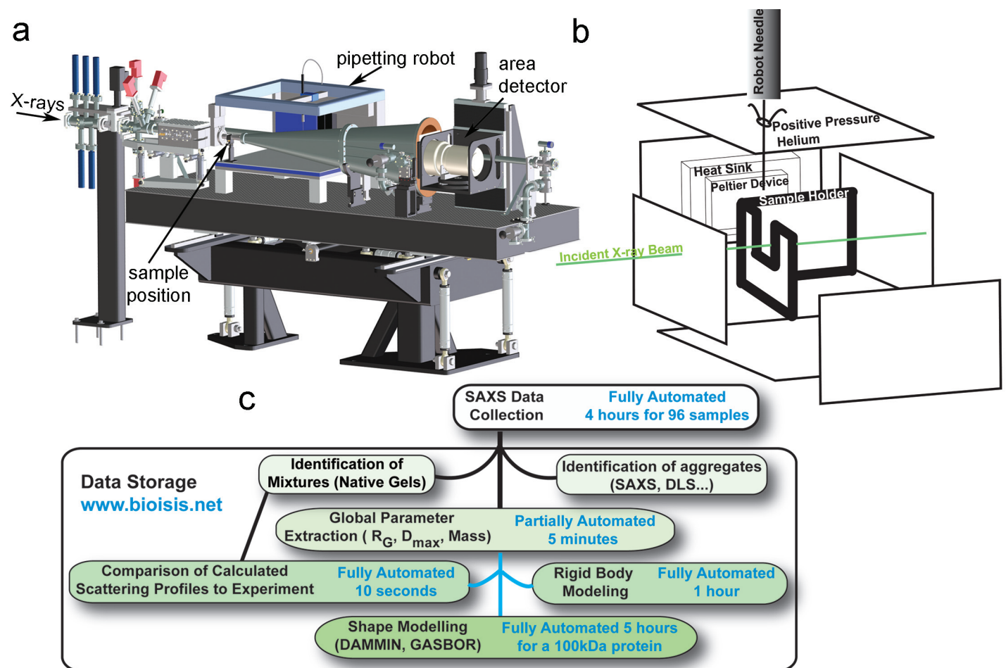
Figure 1. Proteomics-level SAXS platform and pipeline. (a) Configuration of the SAXS endstation shows X-ray beam path, sample position, pipetting robot, and area detector. (b) Schematic of the sample area showing how the sample is loaded by the robot into a temperature-controlled cell. Positive helium pressure reduces air scatter and oxidative damage. (c) SAXS analysis tree for rapid and robust data processing and analysis. Proteins are first categorized as aggregated, mixtures (based on native gel electrophoresis), or mono-disperse samples. For monodisperse samples, SAXS data next defines global solution structural parameters radius of gyration, maximum dimension, and calculated mass ( Table 1 ). Sequence-based homology search discovers existing structures that can be used to analyze both mixtures and mono-disperse samples. Approximate time scales are noted in each step. Perl scripts are used to collect information and begin processes with paths marked in blue. Here we have primarily relied on programs designed by Bio-SAXS Group at EMBL Hamburg 26 . Both primary data and derived shapes are stored at the BioSis internet accessible utility.
