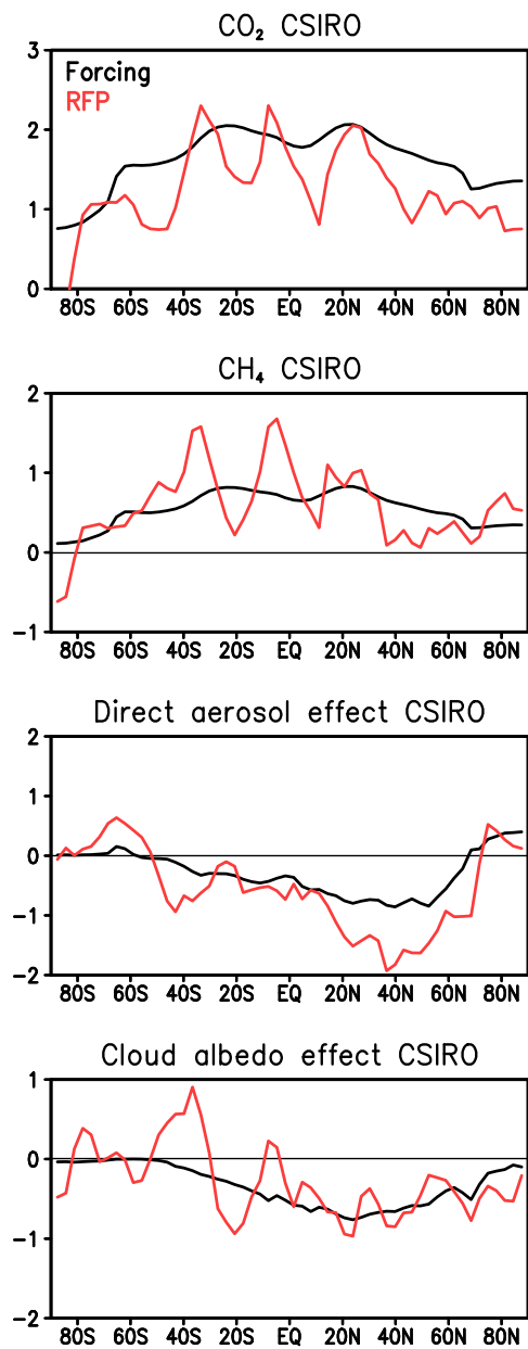
Fig. 6. Annual zonal means of F vs. RFP [ \text{W m}^{-2} ] for the different forcing agents from the CSIRO GCM
