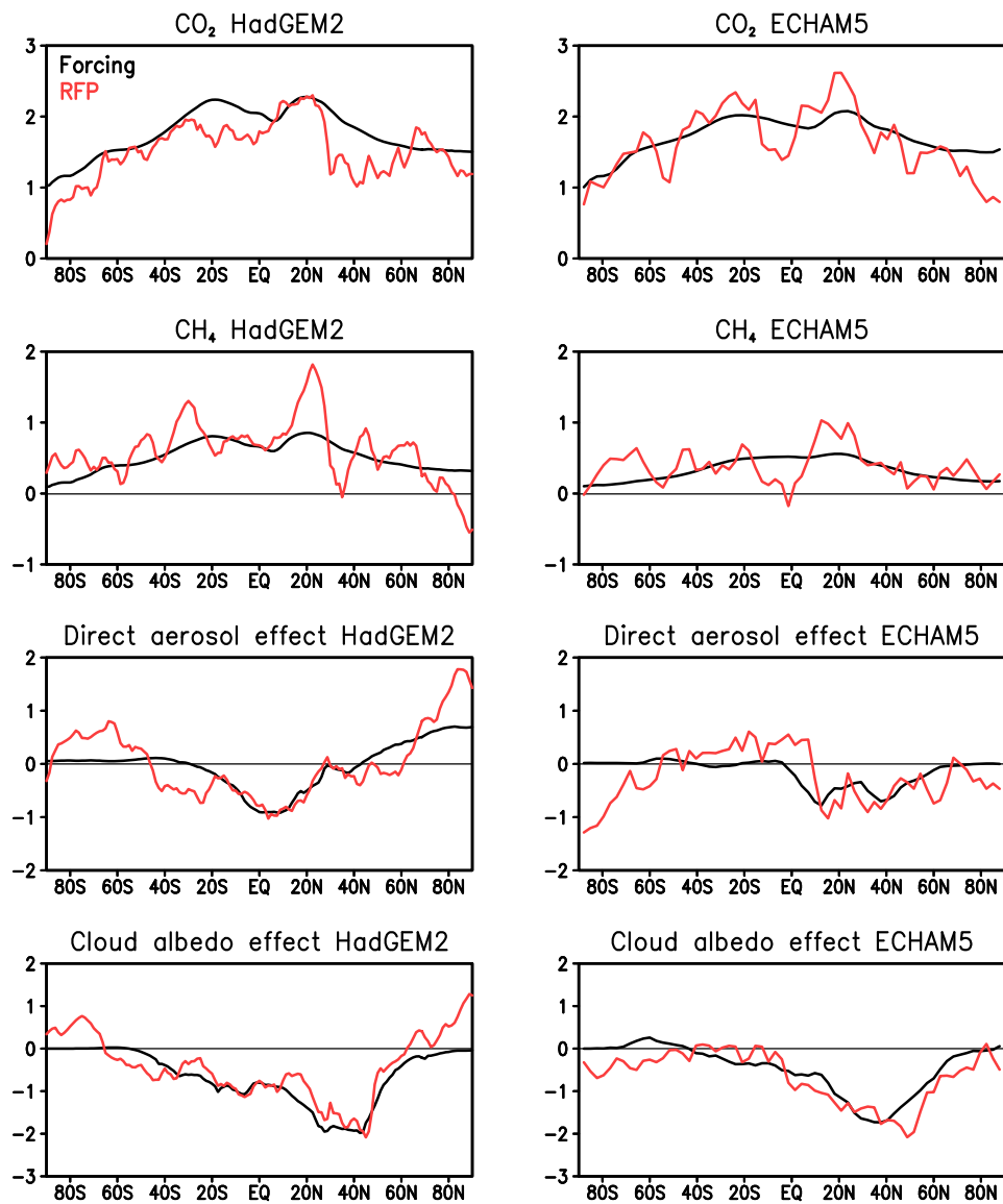
Fig. 4. Annual zonal means of F vs. RFP [ \text{W m}^{-2} ] for the different forcing agents from the HadGEM2 and ECHAM5 GCMs
