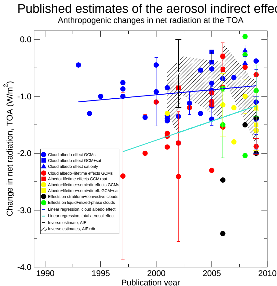
Fig. 1. Model, satellite and inverse estimates of the aerosol indirect effects over the last two decades. Per method or effects considered, each symbol represents one published estimate (one paper one vote). Blue represents estimates of the cloud albedo effect from GCMs (circles), GCMs combined with satellite measurements (squares) and satellite only (triangles). Red represents estimates of both the cloud albedo and cloud lifetime effect from GCMs (circles) and GCMs combined with satellite estimates (squares). The yellow circle represents an estimate of the cloud albedo, lifetime, direct and semi-direct effects. Black circles represent the aerosol effects on stratiform and convective clouds and green circles represent estimates of aerosol effects on liquid and mixed-phase clouds. The black stippled area refers to inverse estimates. In case of multiple estimates per paper, the vertical bars denote the standard deviation. See supplement for the individual papers, from which the estimates are obtained.
