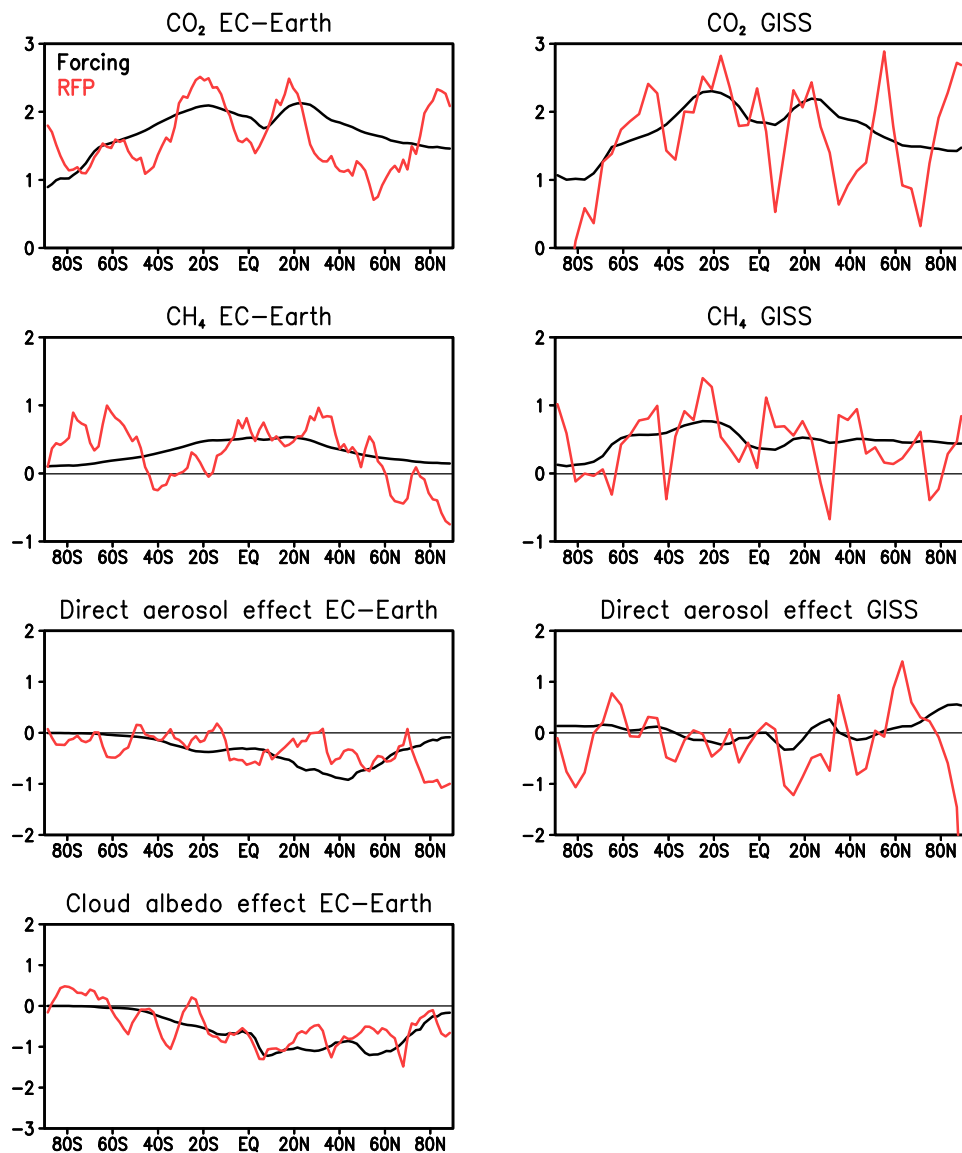
Fig. 5. Annual zonal means of F vs. RFP [ \text{W m}^{-2} ] for the different forcing agents from the EC-Earth and GISS GCMs
