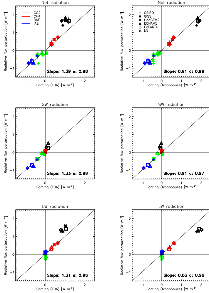
Fig. 2. Net, shortwave and longwave radiative flux perturbation versus TOA and tropopause forcing, respectively, from five GCMs. Vertical bars denote the interannual standard deviation in the radiative flux perturbation calculations.
