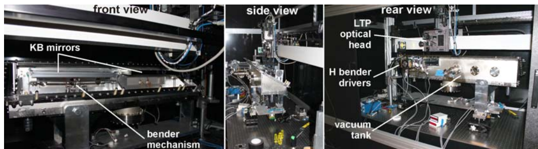
Figure 1: Bendable KB mirrors used at the SLAC/FEL AMO beamline. Two mirrors with 400 mm long substrates are shown in a vacuum tank on the ALS Long Trace Profiler optical table to be characterized and adjusted to the elliptical shapes optimized for three different focus distances.
