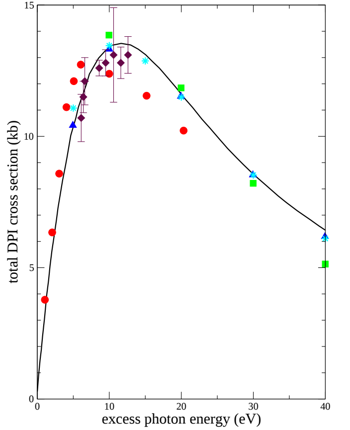
FIG. 3: (Color online) Total DPI cross section from beryllium at various energies. Stars: present results, solid curve: polynomial fit to RMPS calculation [13] of Griffin, et. al. , solid circles: CCC results of Kheifets and Bray [9], solid squares: TDCC results of Colgan and Pindzola [10], solid triangles: B -spline results of Laulan and Bachau [12], solid diamonds with error bars: experimental measurements of Wehlitz, et. al. [16]. 1 \text{ kb} = 10^{-21} \text{ cm}^2 .
