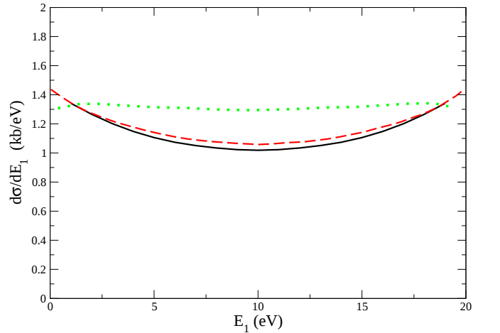
FIG. 4: (Color online) Single differential cross section (SDCS) results for DPI of beryllium at 20 eV excess photon energy. Solid curve: present results; dashed curve: results of Colgan and Pindzola [10]; dotted curve: HRM-SOW results of Citrini, et. al. [11].
