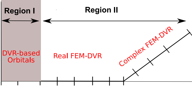
FIG. 1: (Color online) Sketch of hybrid basis constructed from DVR-based orbitals and the primitive Finite-Element Discrete Variable Representation
