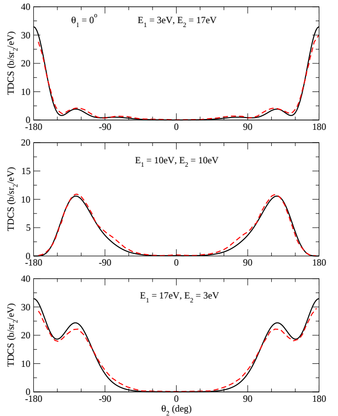
FIG. 6: (Color online) Triply-differential cross section (TDCS) results for DPI of beryllium at 20 eV excess photon energy. The angle of the first electron is fixed along the polarization direction \theta_1 = 0^\circ . Each panel displays results as the energy sharing is varied: from top to bottom, the fixed electron carries 15%, 50% and 85% of the available energy, respectively. Solid curve: present results; dashed curve: results of Colgan and Pindzola [10].
