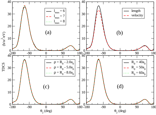
FIG. 2: (Color online) Convergence tests for DPI of beryllium. The TDCS above were calculated with one outgoing electron fixed with 65% energy sharing of 20 eV available excess energy at angle \theta_1 = 20^\circ . Clockwise from upper-left panel show (a) convergence with respect to the angular expansion basis l_{\max} , (b) gauge representation of the dipole operator, (d) size of the purely-real ECS radial grid R_0 , and (c) extraction radius \rho for evaluation of the DPI partial-wave amplitudes. Cross section in units of barns (b) per eV per steradian (sr). 1 \text{ b} = 10^{-24} \text{ cm}^2 . R_0 and \rho in units of a_0 . 1a_0 = 0.529 \times 10^{-8} \text{ cm} .
