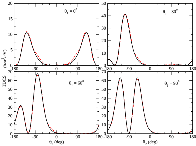
FIG. 5: (Color online) Triply-differential cross section (TDCS) results for DPI of beryllium at 20 eV excess photon energy. The electrons share equal amounts of energy E_1 = E_2 = 10 eV. Each of the panels shows a different fixed value of the direction of the first electron \theta_1 . Solid curve: present results; dashed curve: results of Colgan and Pindzola [10].
