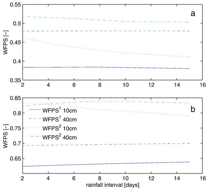
Fig. 4. 30-day mean water filled pore space (WFPS) at 10 and 40 cm depth for (a) sandy loam and (b) clay loam soils as a function of rainfall intervals. \text{WFPS}^1 and \text{WFPS}^2 represent WFPS from 1.5 \text{ cm month}^{-1} scenario and 15 \text{ cm month}^{-1} scenario, respectively.
