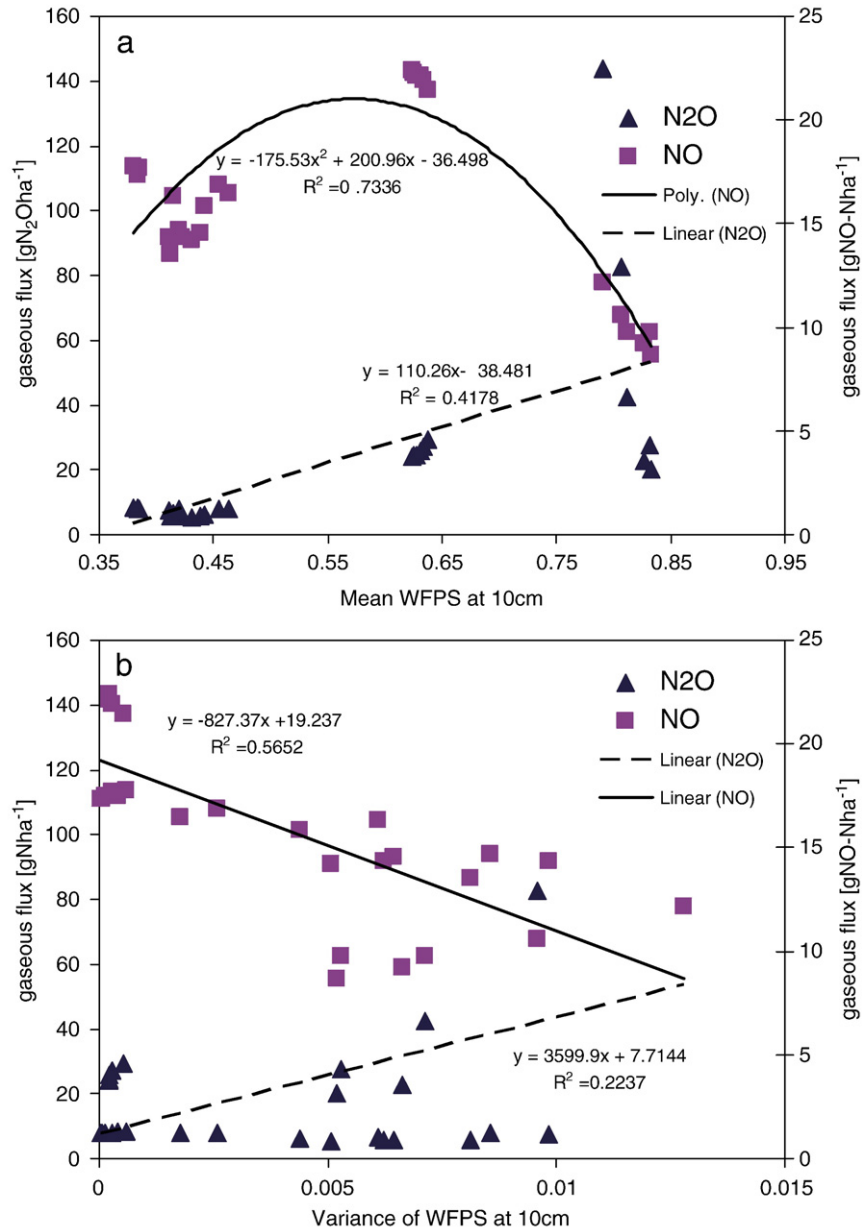
Fig. 7. Relationships between \text{NO} and \text{N}_2\text{O} fluxes and (a) mean soil WFPS at 10 cm depth and (b) variance of soil WFPS at 10 cm depth. These relationships are based on all simulation results combining three treatment variables.
