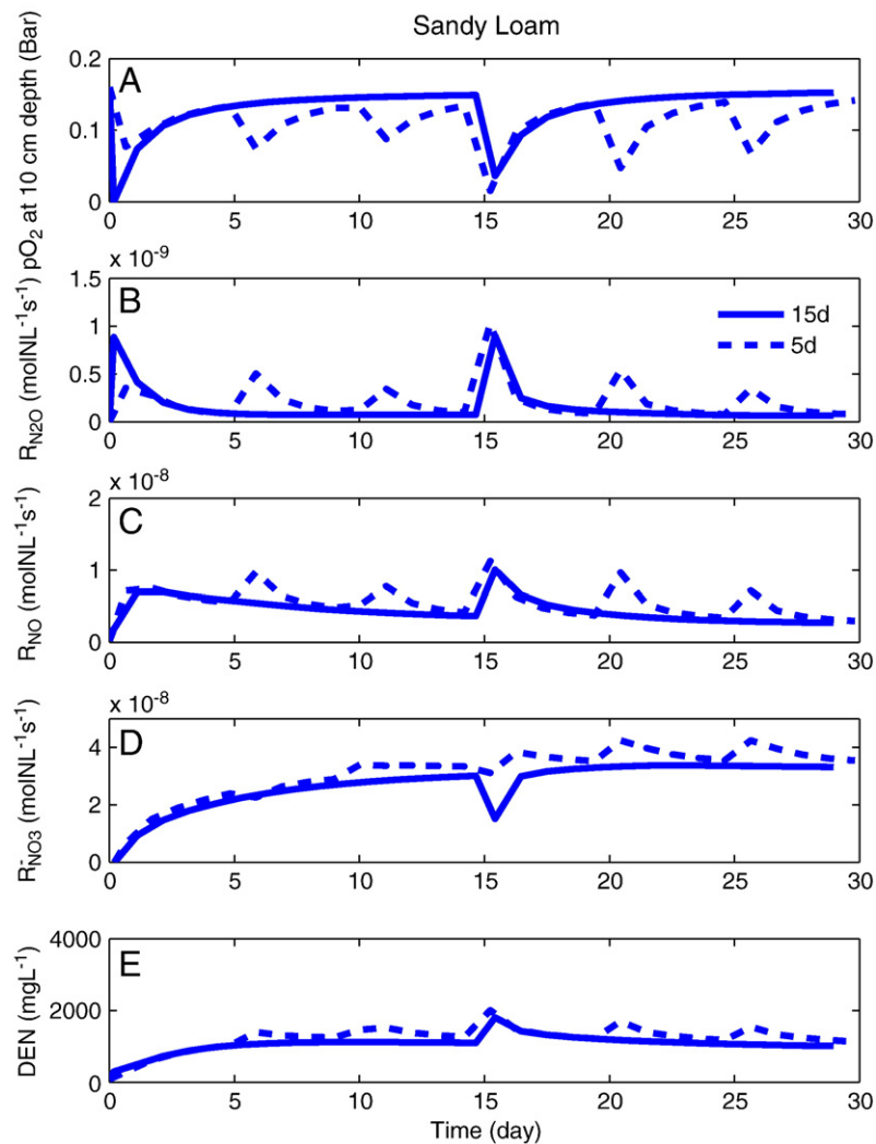
Fig. 5. Time series of (A) soil oxygen partial pressure at 10 cm depth and depth integrated (B) net \text{N}_2\text{O} , (C) NO, (D) \text{NO}_3^- production rates, and (E) denitrifier (DEN) concentration from sandy loam soil for 5-day and 15-day precipitation intervals.
