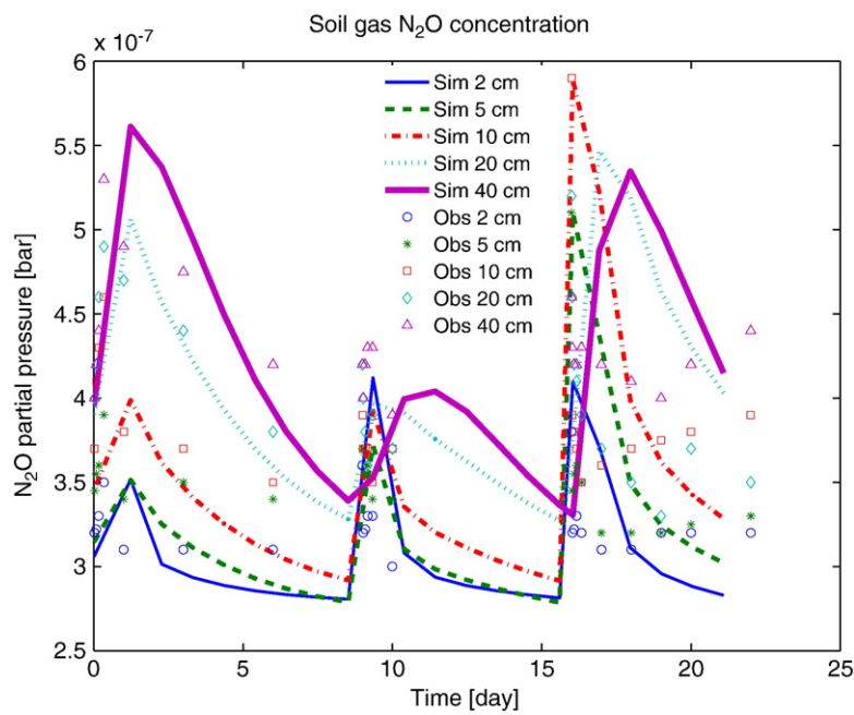
Fig. 3. Observed and simulated soil \text{N}_2\text{O} partial pressure (bar) profiles at the Costa Rican Cordillera Central site in response to three water additions on days 0, 9, and 16.
