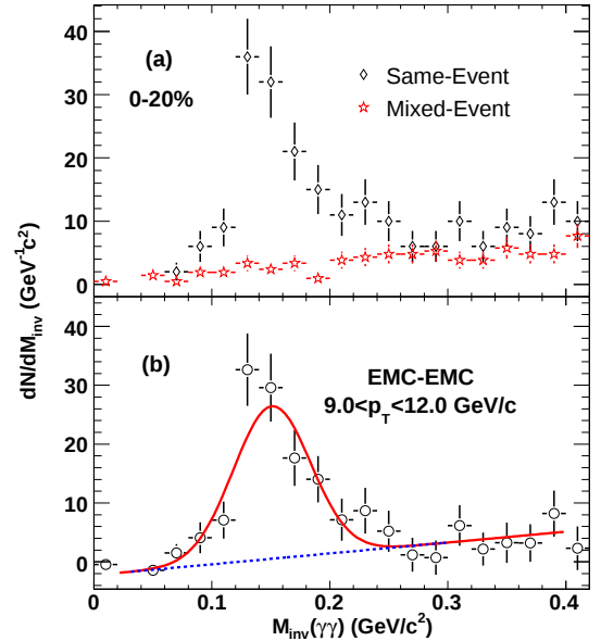
FIG. 2: The di-photon invariant mass distributions using the EMC-EMC method in 0-20% Au+Au collisions at \sqrt{s_{NN}} = 200 GeV. The solid line is a fit result of a Gaussian peak plus a background function. The residual background is shown as a dotted line. Panels (b) is the distribution after mixed-event background subtraction from panel (a).
