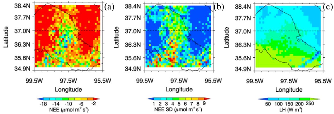
Figure 8. For noon, April 15, 2003: (a) NEE (b) Fractional-cover-weighted standard deviation of NEE; and (c) LH flux. NEE spatial variation (SD) within the 10 km gridcells at a particular time can be larger than the mean in the gridcell, while LH fluxes are typically much less heterogeneous than NEE.
