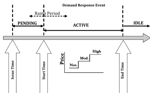
Figure 5 Automated critical peak pricing (Auto-CPP) mapping on OpenADR specification
