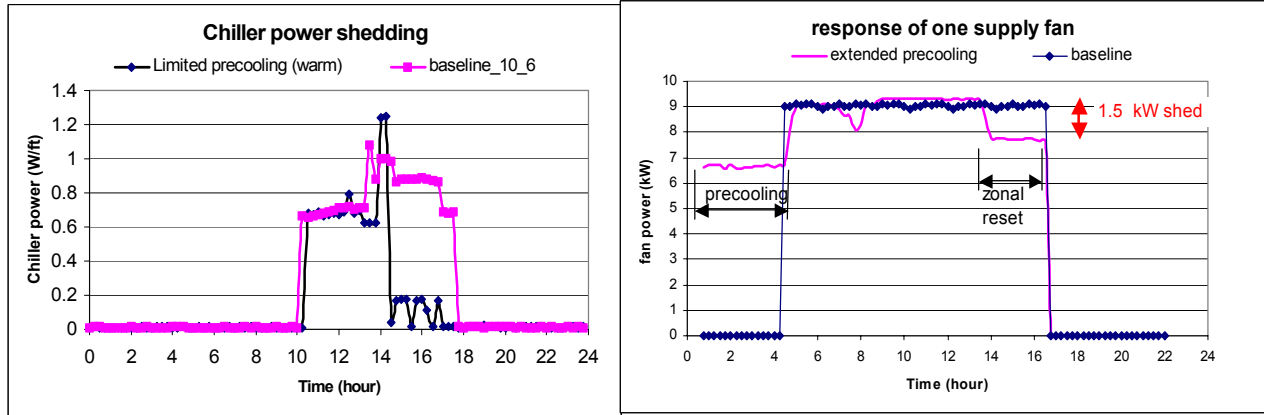
Figure 9 Chiller Power in Pre-Cooling Tests
