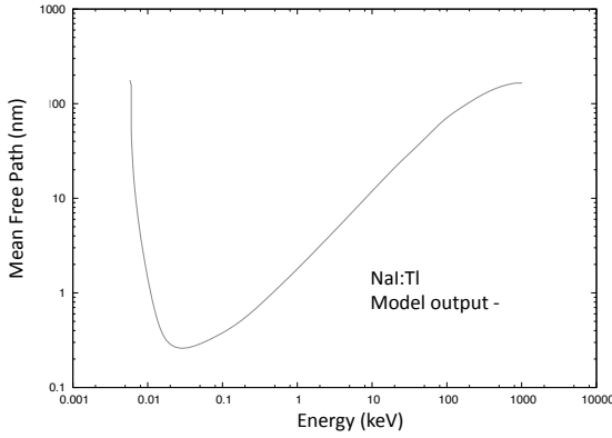
Fig. 3. Mean Free Path as a function of the incident electron energy calculated for NaI:TI
