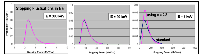
Fig. 6: Calculations of Landau distributions for three electron energies in \text{NaI} , with and without inclusion of the c term (using c=0 and c=2.8 ).
