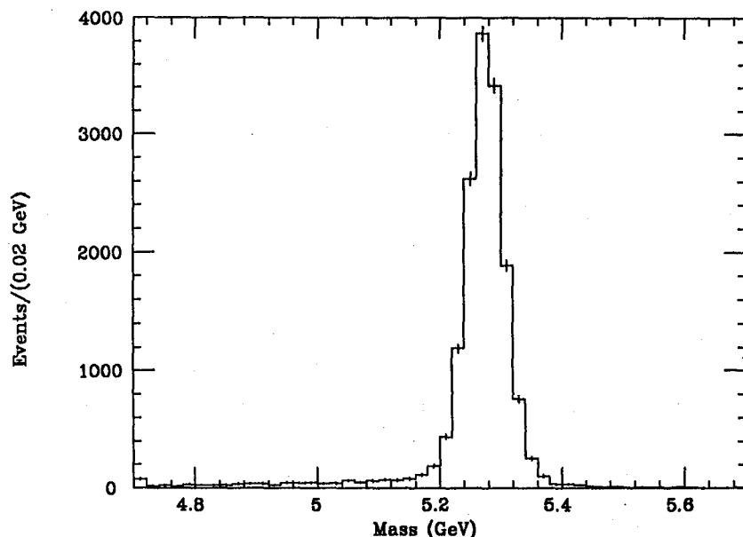
Figure 5.2. Invariant mass distribution for J/\psi K_S^0 candidates in events in which one B decays to J/\psi K_S^0 .
