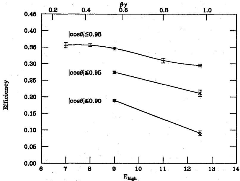
Figure 5.6 The efficiency for reconstructing B \rightarrow J/\psi K_S^0 and tagging the other B , as a function of boost and low-angle cut-off. E_{\text{high}} is the energy of higher energy beam.
