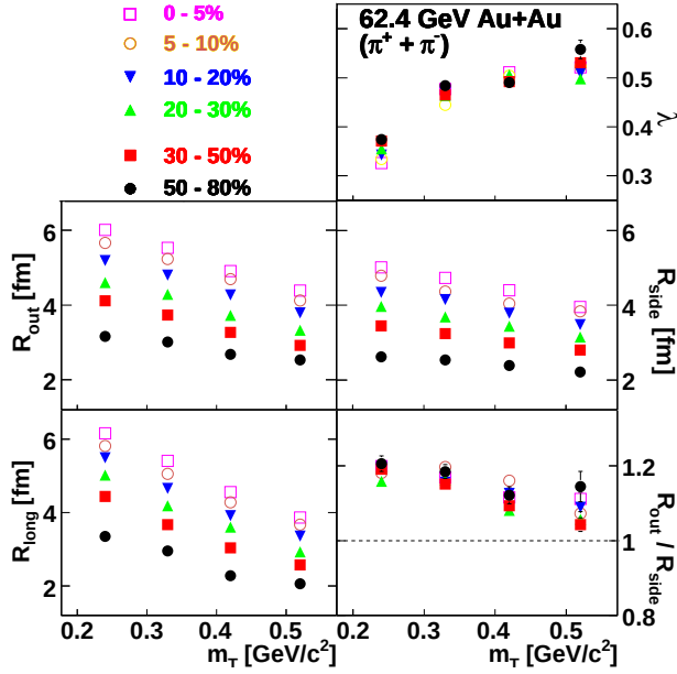
FIG. 1: (Color Online) The femtosopic parameters vs. m_T for 6 different centralities for Au+Au collisions at \sqrt{s_{NN}} = 62.4 GeV. Only statistical errors are shown. The estimated systematic errors are less than 10% for R_{out} , R_{side} , R_{long} , \lambda in all centrality and k_T bins.
