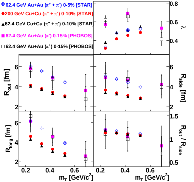
FIG. 7: (Color Online) The comparison of femtoscopic measurements of STAR Cu+Cu collisions at \sqrt{s_{NN}} = 200 and 62.4 GeV and Au+Au collisions at \sqrt{s_{NN}} = 62.4 GeV. Only statistical errors are shown for STAR results. The estimated systematic errors for STAR results are less than 10% for R_{out} , R_{side} , R_{long} , \lambda in all centrality and k_T bins. The PHOBOS results [50] for positive and negative pions in Au+Au collisions at \sqrt{s_{NN}} = 62.4 GeV are compared with STAR results.
