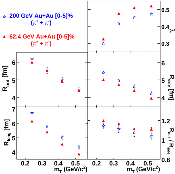
FIG. 2: (Color Online) The comparison of femtosopic measurements of Au+Au collisions at \sqrt{s_{NN}} = 200 GeV and 62.4 GeV for 0-5% most central events. Only statistical errors are shown for Au+Au collisions at \sqrt{s_{NN}} = 62.4 GeV. The estimated systematic errors for Au+Au collisions at \sqrt{s_{NN}} = 62.4 GeV are less than 10% for R_{out} , R_{side} , R_{long} , \lambda in 0-5% most central events and all k_T bins. The 200 GeV results are from [17].
