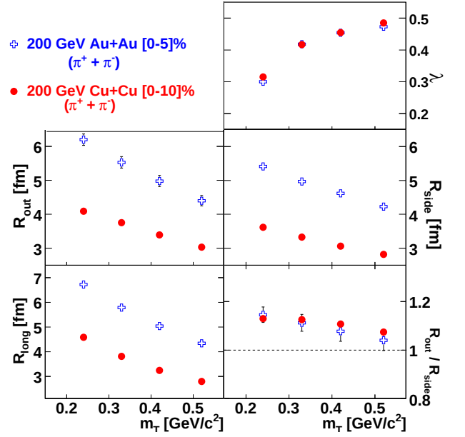
FIG. 6: (Color Online) The comparison of system size dependence in femtoscopic measurements of STAR Au+Au and Cu+Cu collisions at \sqrt{s_{NN}} = 200 GeV. Only statistical errors are shown for Cu+Cu collisions at \sqrt{s_{NN}} = 200 GeV. The estimated systematic errors for Cu+Cu collisions at \sqrt{s_{NN}} = 200 GeV are less than 10% for R_{out} , R_{side} , R_{long} , \lambda in 0-10% most central events and k_T bins. The Au+Au results are from [17].
