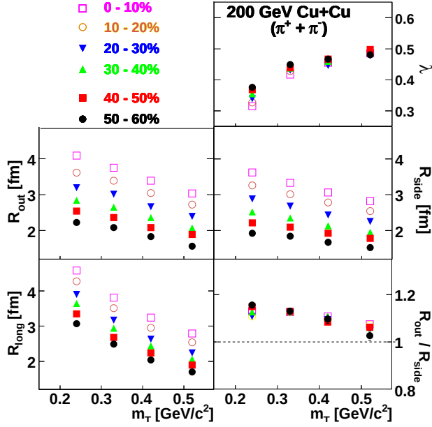
FIG. 5: (Color Online) Femtoscopic parameters vs. m_T for six centralities for Cu+Cu collisions at \sqrt{s_{NN}} = 200 GeV. Only statistical errors are shown. The estimated systematic errors are less than 10% for R_{out} , R_{side} , R_{long} , \lambda in all centrality and k_T bins.
