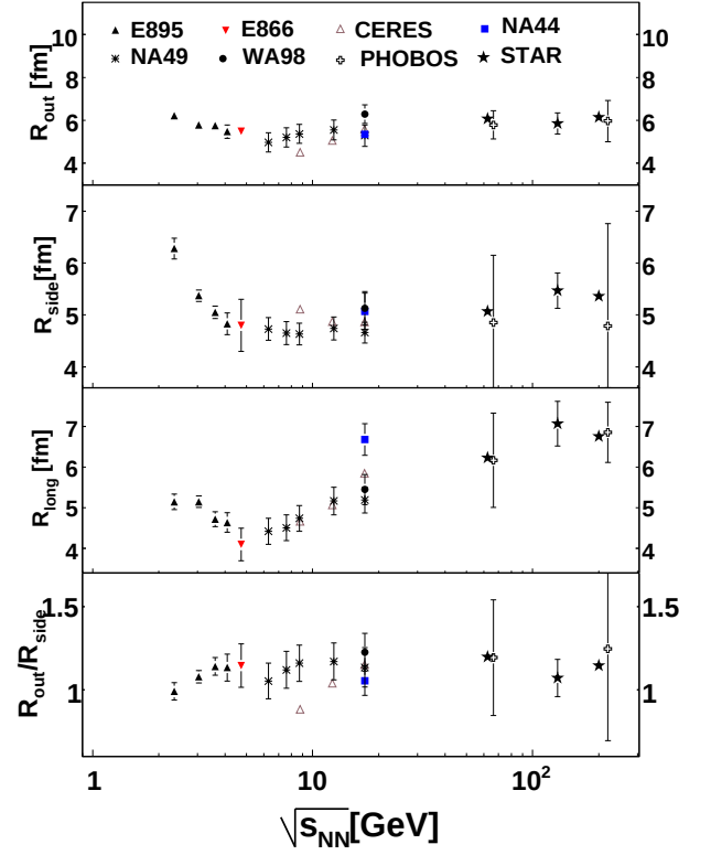
FIG. 3: (Color Online) The energy dependence of femtosopic parameters for AGS, SPS and RHIC from Refs. [14, 17, 50, 51, 52, 53, 54, 55, 56, 57]. Energy dependences of pion femtosopic parameters for central Au+Au, Pb+Pb and Pb+Au collisions are shown for mid-rapidity and \langle k_T \rangle \sim 0.2-0.3 GeV/c. Error bars on NA44, NA49, CERES, PHOBOS and STAR results at \sqrt{s_{NN}} = 130 and 200 GeV include systematic uncertainties; error bars on other results are statistical only. Only statistical errors are shown for Au+Au collisions at \sqrt{s_{NN}} = 62.4 GeV; the estimated systematic errors are less than 10% for R_{out} , R_{side} , R_{long} . The PHOBOS results from [50] for \sqrt{s_{NN}} = 62.4 and 200 GeV are slightly shifted horizontally for visual clarity.
