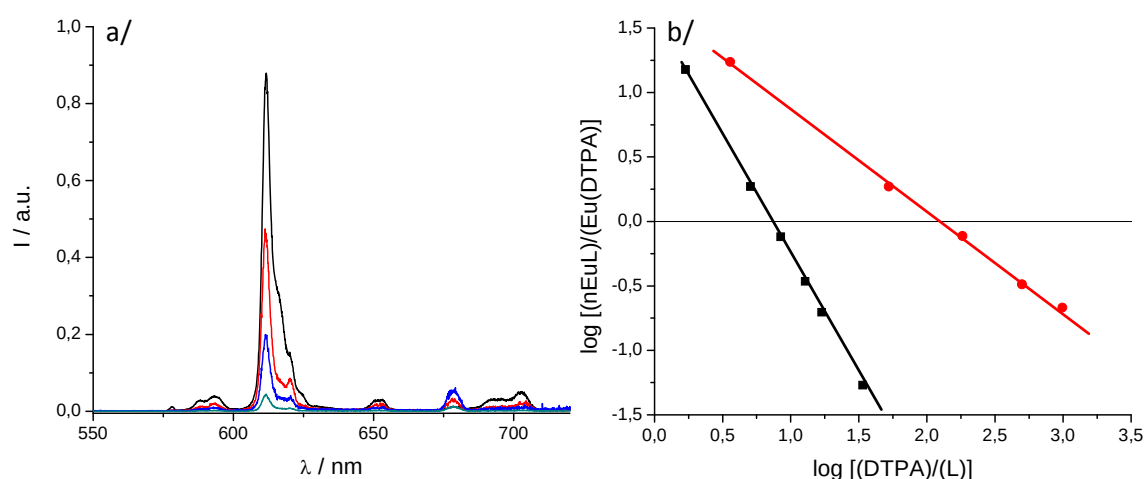
Figure 1. a/ Luminescence spectrum showing the typical decrease of luminescence intensity upon addition of DTPA; b/ DTPA competition batch titration of [Eu(3LI-bis-LYS-1,2-)]
