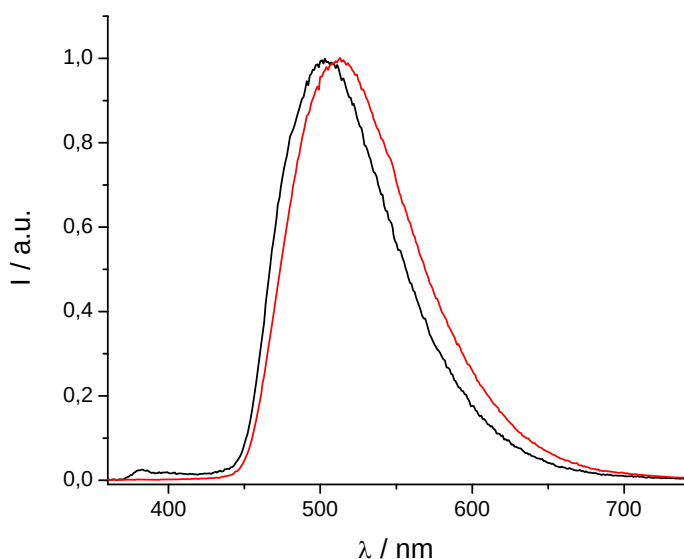
Figure 3. Triplet excited state emission spectra for [Gd(3LI-bis-LYS-1,2-HOPO)] - (—) and [Gd(H(2,2)-1,2-HOPO)] - (—) in solid matrix (77K, 1:4 (v/v) MeOH:EtOH) ( \lambda_{\text{ex}} = 340nm).
