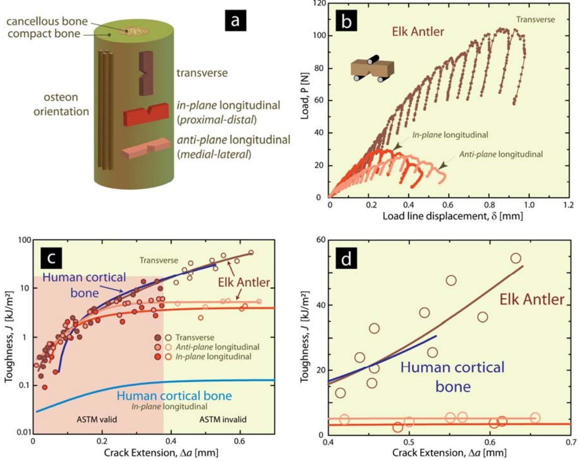
Fig. 3. The schematic (a) shows the structure of antler bone, as well as the three anatomical orientations that the specimens were taken from the compact bone. (b) Typical load vs. load-line displacement curve obtained during R-curve testing for the transverse, in-plane longitudinal, and anti-plane longitudinal orientation of antler compact bone. Each partial unloading event during the test corresponds to a data point in (c). (c) Full J_R(\Delta a) resistance curves for stable ex situ crack extension in hydrated antler compact bone tested in transverse, in-plane longitudinal, and anti-plane longitudinal orientations. (d) expansion of (c) showing J_R(\Delta a) resistance curves at larger crack extension ( \Delta a > 0.4 mm). The R-curves for short crack lengths ( \Delta a \approx 0.6 mm) are compared with data taken from human cortical bone in both transverse and in-plane longitudinal orientations of the humerus. Data for human cortical bone were adapted from Ref. [17]. In the transverse orientation, fracture toughnesses, J , of antler compact bone were recorded at nearly \sim 60 kJ/m 2 , almost two times higher than the critical toughness value, J_c , of human cortical bone ( J_c \approx 30 kJ/m 2 ). The validity of these data points is defined by the measurement capacity of each specimen in accordance with the ASTM standard [13]. The circles in (c) and (d) correspond to data points for antler bone.
