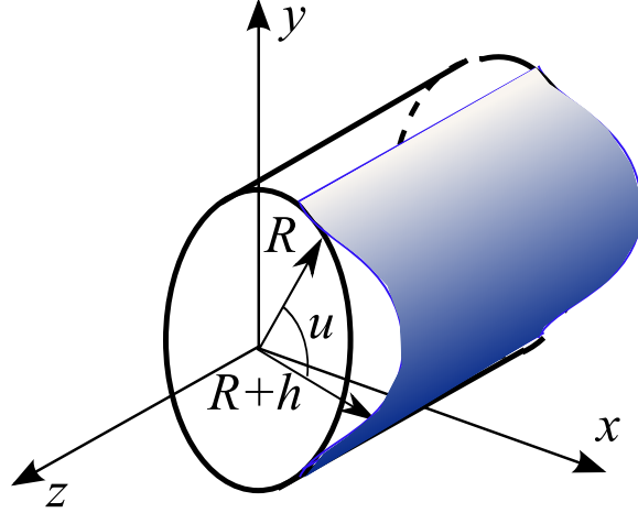
FIGURE 3. A liquid film on a cylindrical surface
