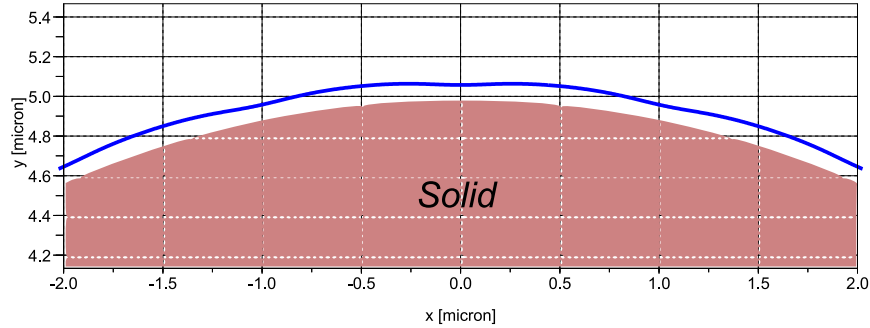
FIGURE 7. A periodically oscillating solution to the AYLE. The amplitude of the thickness variation has been amplified for visualization.
