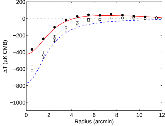
Fig. 4.— Radial profile of Sunyaev-Zel'dovich effect in the Bullet cluster compared to the best-fit \beta model. Points with error bars are the SZE data binned in 1' radial bins, from the non-source-masked map, ( \mathcal{M} , filled circles) and the source-masked map (open circles). The lines show the radial profile of the best-fit \beta model, unfiltered ( \mathcal{B} , blue dashed line) and after convolving with the instrument beam and non-source-masked data reduction filters ( \mathcal{B}' , red solid line). The non-source-masked map radial profile is reasonably well fit by the filtered \beta model. The source-masked map preserves signal on larger spatial scales than the non-source-masked map, but still attenuates signal on scales exceeding the 4.75' radius of the source masking. The source-masked data thus have a lower signal amplitude when compared with the unfiltered \beta model, as expected. See text for details.
