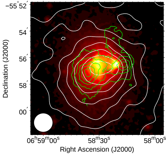
Fig. 5.— The SZE map of the Bullet system from this work, in white contours, overlaid on an X-ray map from XMM observations. The green contours show the weak lensing surface mass density reconstruction from Clowe et al. (2006). The SZE contour interval is 100 \mu\text{K}_{\text{CMB}} .
