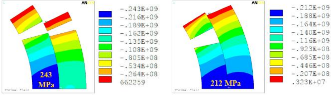
Figure 2: Azimuthal stress distribution due to Lorentz forces at 200 T/m in an infinitely stiff structure with sliding between layers for two 134 mm aperture cross-sections. Left: F_{\theta} L_1 = -3.58 \text{ MN/m} F_{\theta} L_2 = -2.46 \text{ MN/m} – Right: F_{\theta} L_1 = -2.7 \text{ MN/m} F_{\theta} L_2 = -3.4 \text{ MN/m}
