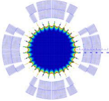
Figure 2: HQ 114 mm aperture cross-section designed by Vadim Kashinkhin, FNAL
