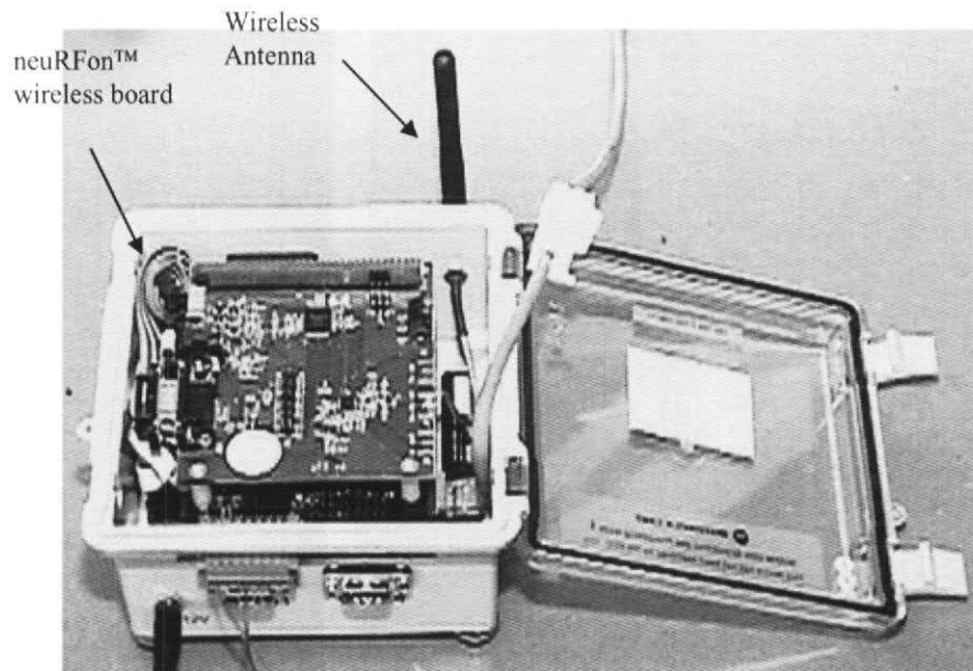
Figure 5. The Motorola neuRFon™ wireless communication board displayed on the prototype WiSHM system.
