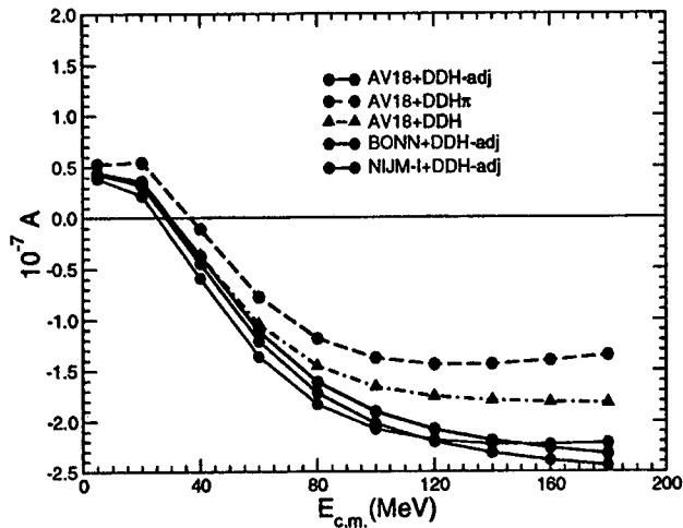
Fig. 3. Longitudinal asymmetry in np polarized scattering for various weak interaction models (see text).
