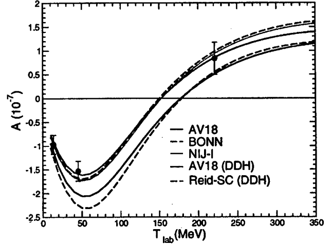
Fig. 2. Comparison of original and adjusted DDH models with pp TRIUMF measurements.
