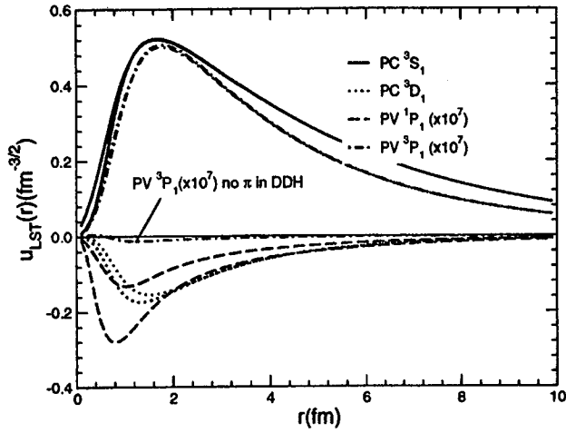
Fig. 1. PV components of the deuteron, with and w/o pion coupling in DDH.
