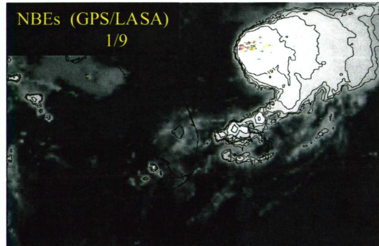
Figure 2. Temporal evolution of Tropical Storm Edouard on Sept. 3, 2002 from 10:30 UT through 12:30 UT in 0.5-hour increments. LASA-detected lightning events are identified as CGs (green), NBEs (red) and unknown (yellow). Those NBEs also detected by LASA are shown in blue. Lightning polarities are indicated by “-” or “+” symbols.
