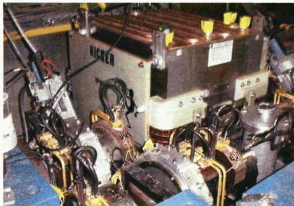
Figure 4: The IPF kicker magnet as installed in the LANSCE transition region. Upstream end of the magnet is to the left.
