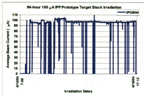
Figure 7: Average beam current data taken during a 96-hr 100\text{-}\mu A irradiation of an IPF prototype target stack.
