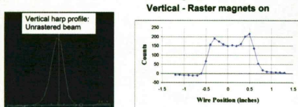
Figure 6: Vertical beam profile without and with rastering.
