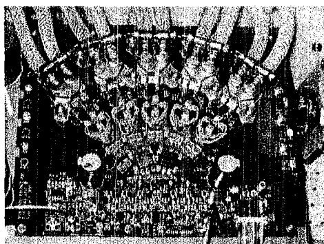
Figure 7 One-half of the MEBT chopper pulser output switch assembly
