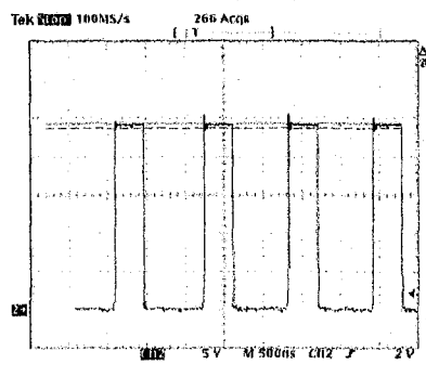
Figure 8. String of four pulses (out of ~1000 during a 1-ms SNS macropulse, repeated at 60 Hz).
