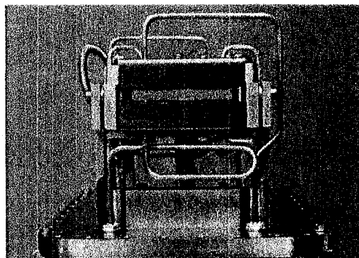
Figure 2. End view of the chopper structure
