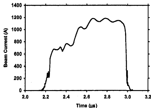
Figure 6. Electron beam current at accelerator exit.
