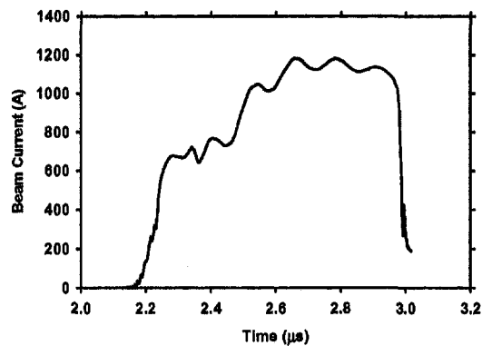
Figure 5. Electron beam current at BCUZ exit.
