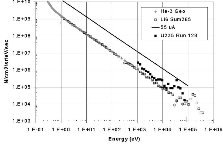
Figure 1. Surface current for FP14 at the Lujan Center, measured at 55 \mu A proton current. The predicted surface current is shown as the solid line.
