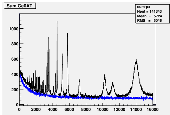
Figure 2. Time of flight spectrum for ^{151}\text{Sm}(n,\gamma) . The contribution from a blank Ti foil sandwich is shown as the smooth gray curve. The time calibration is 100 ns/channel.
