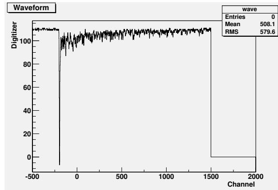
Figure 3. Typical waveform from a completed Ba 2 crystal assembly using a DC-720 1 GHz digitizer. One channel corresponds to 1 ns. The fast and slow components are easily recognized.
