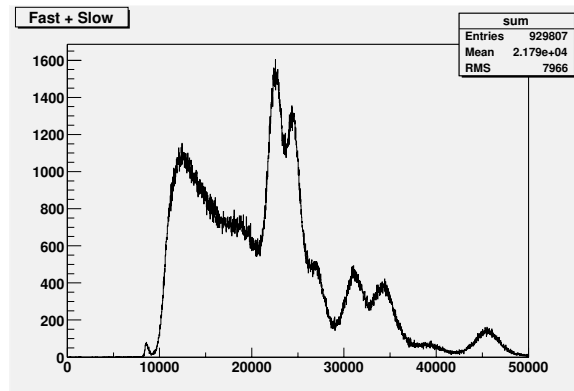
Figure 4. ^{60}\text{Co} spectrum obtained by simply summing waveforms from a 1 GHz digitizer. The peaks from the alpha-decay background in the crystal are readily seen.
