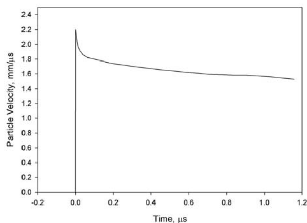
FIGURE 3. DETONATING NM/PMMA INTERFACE PARTICLE VELOCITY PROFILE OBTAINED IN COMMERCIAL GRADE NM USING FABRY-PEROT INTERFEROMETRY. WAVEFORM FROM SHOT 8-294.
