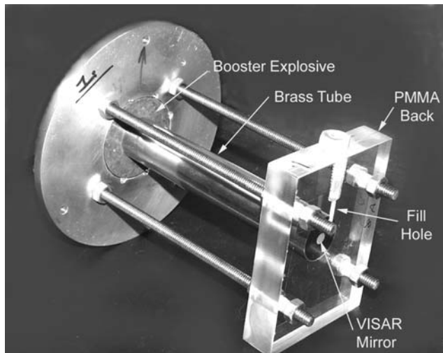
FIGURE 2. OVERALL CONFIGURATION FOR THE NM REACTION ZONE MEASUREMENT EXPERIMENTS. IN THE UPPER LEFT IS THE ALUMINUM TARGET PLATE WHICH IS IMPACTED BY THE GAS-GUN DRIVEN PROJECTILE. THE RESULTING SHOCK THEN INITIATES THE BOOSTER EXPLOSIVE WHICH INITIATES THE NM. THE NM IS CONTAINED IN EITHER A BRASS OR PYREX TUBE. TO THE LOWER RIGHT IS THE PMMA BACK/WINDOW WITH A THIN ALUMINUM LAYER VAPOR PLATED ON THE SIDE NEAR THE NM.
