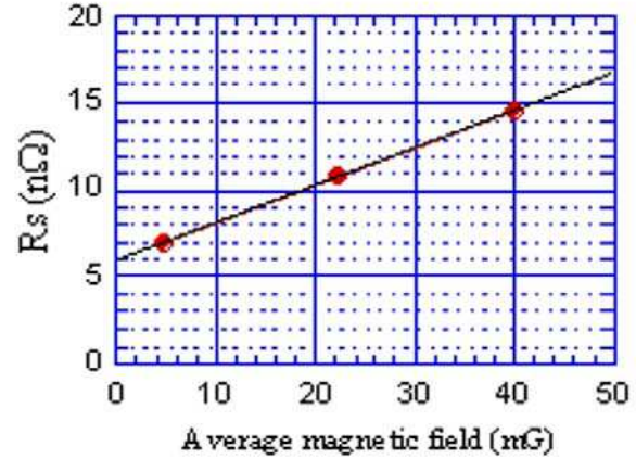
Figure 3: Residual resistance as a function of magnetic field averaged over 5 cells. The sensitivity is calculated to be 0.22 nΩ/mG.
