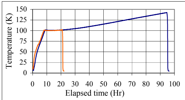
Figure 5: Temperature evolution when the cavity was held at an intermediate temperature. Holding times for the first and second tests were 13 hours at 100 – 102 K and 86 hours at 100 – 142 K, respectively.
