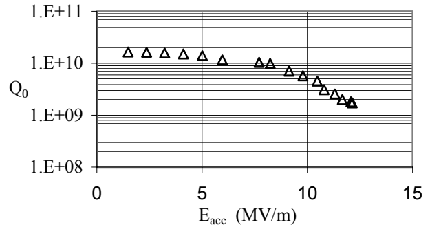
Figure 1: A typical Q - E curve for the APT elliptical cavity developed [3, 5]. E_{peak}/E_{acc} and H_{peak}/E_{acc} are 3.38 and 69.6 Oe/(MV/m), respectively. The limitation in field was field emission and available RF power.
