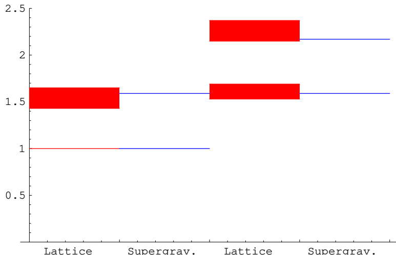
Figure 1: Lattice and supergravity estimates of glueball masses divided by the mass of the 0^{++} . Shown on the left are the first two 0^{++} states; on the right the first two 0^{-+} states.
