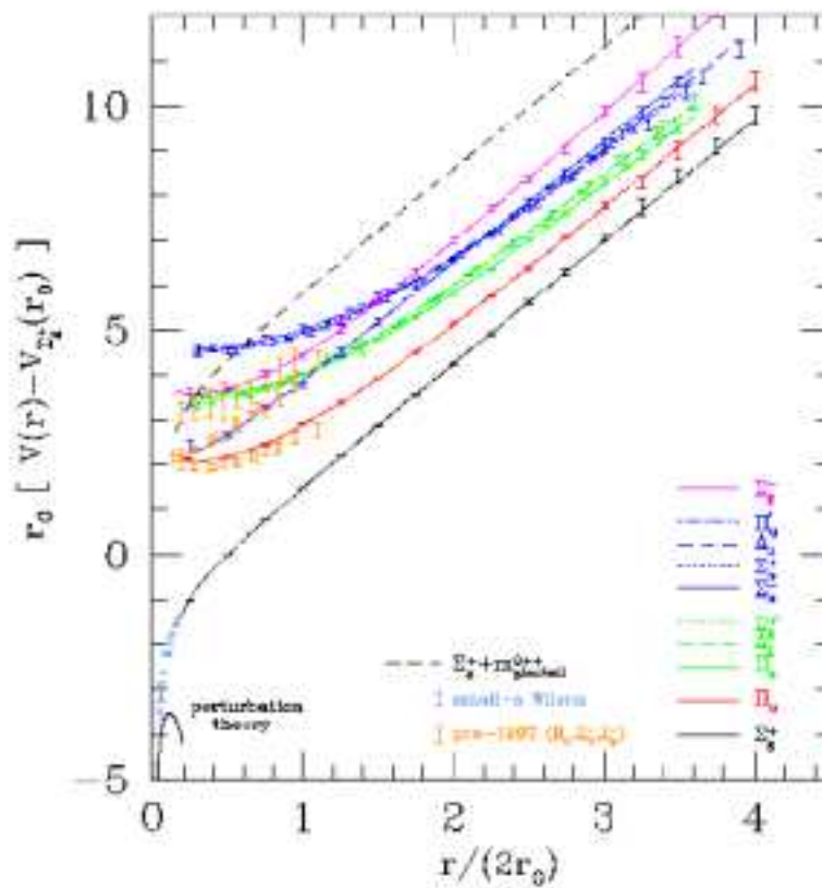
Figure 4: Adiabatic potentials as a function of Q\bar{Q} separation. 33
