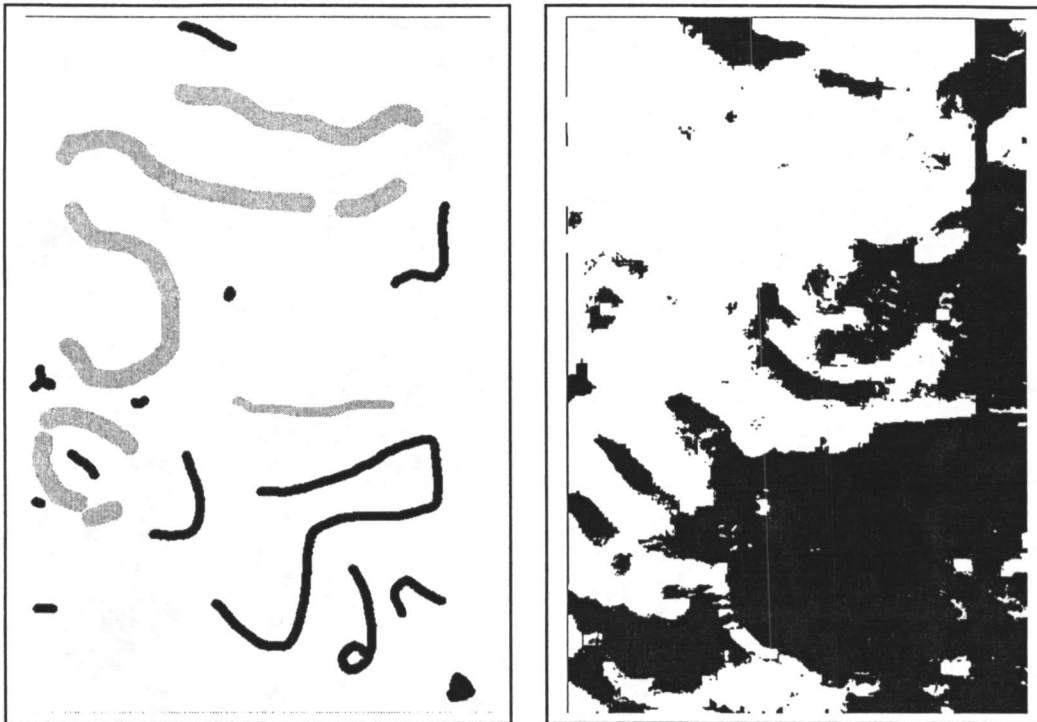
Figure 3. Generic forest feature. Left: Training data provided to GENIE. Black pixels define non-forest training example pixels, and gray pixels define forest example pixels. Right: GENIE's result. Forest was detected in pixels marked in white. Compared to the training data, this result achieved a detection rate of 99.4% and a false alarm rate of 0.5%. Outside of the training pixels, performance is qualitatively good, based on comparison to existing, manual land cover maps.
