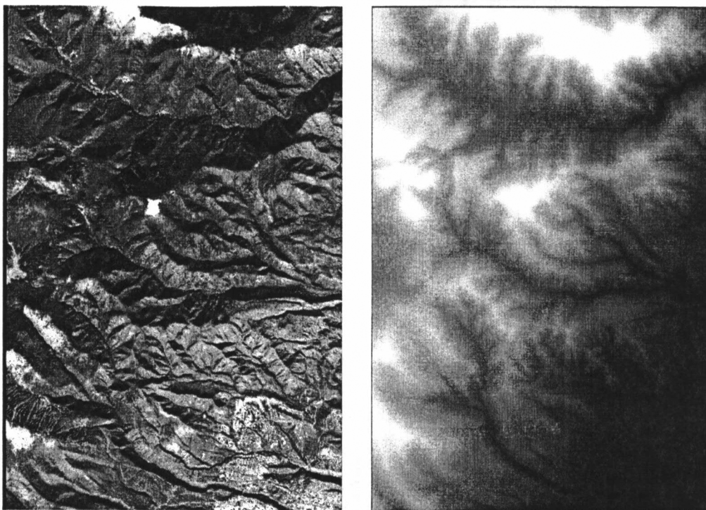
Figure 1. Region of interest. The left panel shows the part of the Jemez Mountains North-west of the town of Los Alamos. This is a grayscale representation of a color-infrared slice through the Multispectral Thermal Imager (MTI) image cube (using MTI bands D-C-B). Solar angle is such that north-facing slopes appear dark. The right panel shows the matching DEM data which is co-registered and added to the multispectral imagery to form our fused datacube. In the DEM, brighter pixels correspond to higher elevations.
