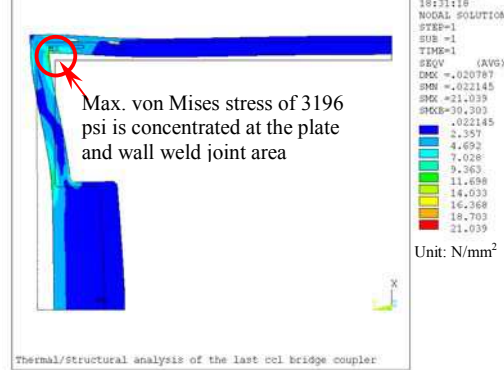
Figure 5: 2-D FEA Model Von Mises Stress Distributions
