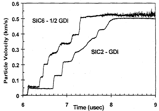
FIGURE 3. Effect of loading rate. Increasing loading rate results in higher peak particle velocity.
