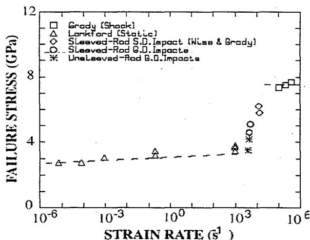
Figure 6. Variation of failure stress with strain rate for Coors AD995. Quasi-static and shock loading experiments are also shown.
