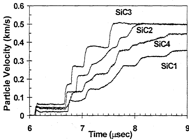
FIGURE 2. Effect of stress and loading rate results in higher peak particle velocity, until a maximum level is achieved.
