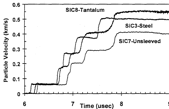
FIGURE 4. Effect of confinement. Confining SiC results in failure at higher stresses because more damage has occurred in the material.
