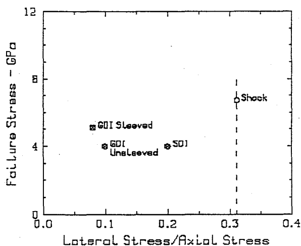
Figure 7. Variation of calculated failure stress as a function of confinement i.e. , the ratio of lateral stress to axial stress.
