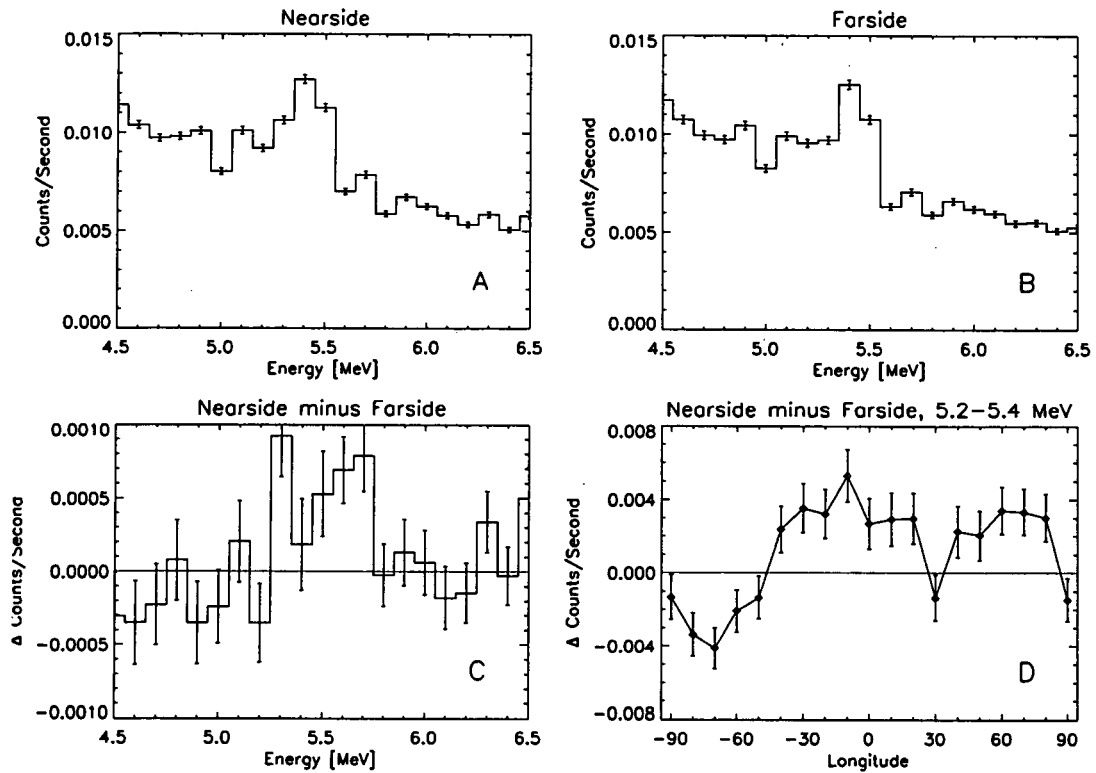
Figure 1. LP APS spectra for the equatorial (a) nearside and (b) farside of the lunar surface. (c) Nearside spectrum minus farside spectrum. (d) Binned nearside minus farside in only the 5.2–5.4 MeV energy range (polonium-210).
