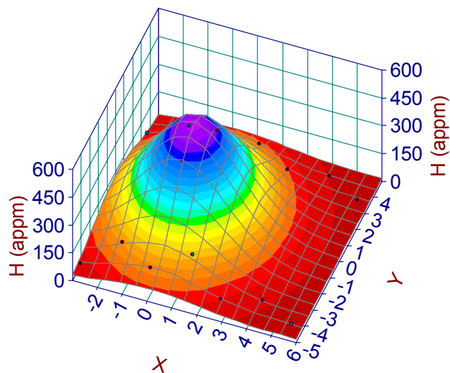
Figure 4. H production for Al6061 in 18A tubes. The foil stack locations are the points distributed above and below the peak.
