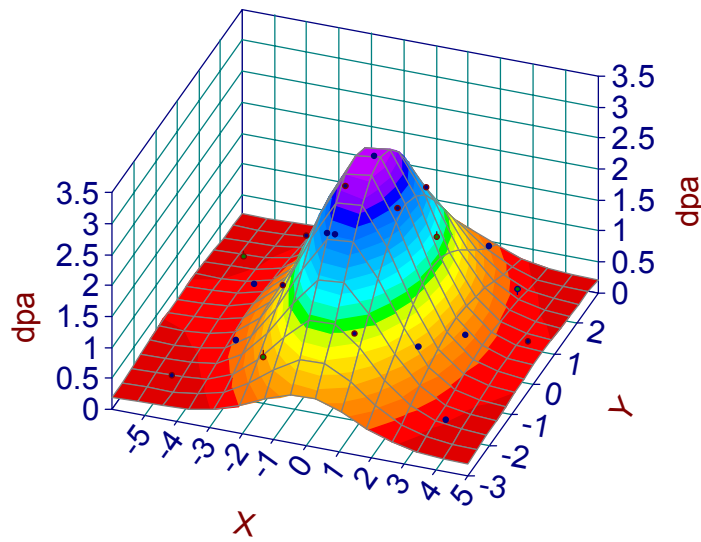
Figure 7. The 316L dpa from tubes in 17A insert from 1998 irradiation. The dots are activation foil locations. The tubes are located in the x direction.
