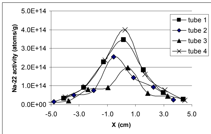
Figure 2. Curves for Al-Na22 activity in foils from "new" 17A.
