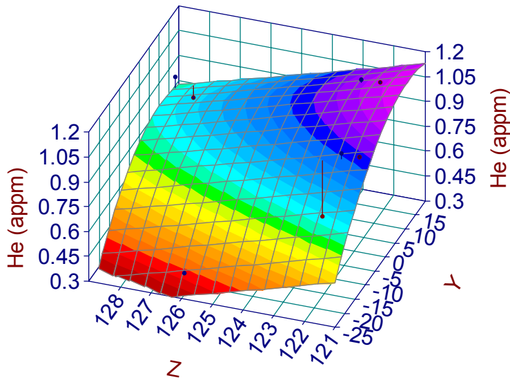
Figure 6. He production (in appm) in Al6061 for neutron furnaces located in off-beam location. There are five furnaces distributed over the Y-Z plane covered by this fit.
