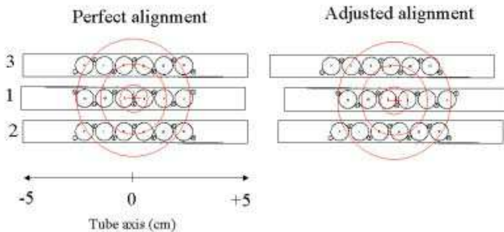
Figure 3. Relative offsets for the tubes and the proton beam – “new” 17A.
