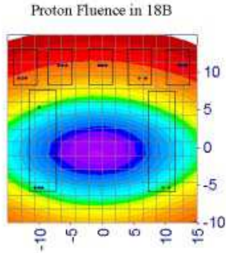
Figure 5. Proton fluence contour plot showing neutron furnaces, foil stacks and distribution of protons around the proton beam. The proton fluence in the furnaces ranged from 2 \times 10^{18} to 1 \times 10^{19} p/cm 2 . In this figure, the peak proton fluence is about 1.34 \times 10^{19} p/cm 2 .
