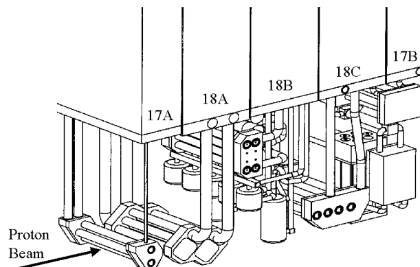
Figure 1. Graphic of the 1996-1997 target configuration in LANSCE Area A-6
