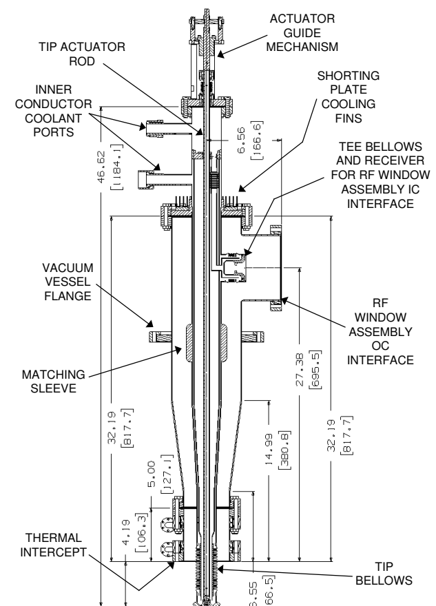
Figure 3: Power coupler schematic (adjustable-tip design)
