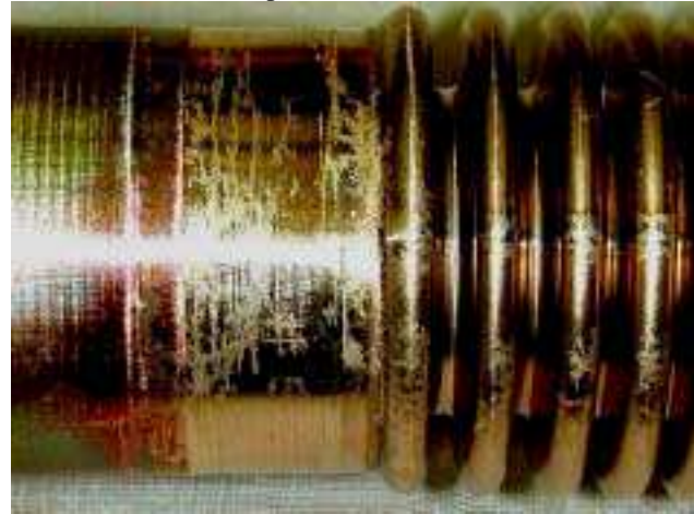
Figure 7: Electronic etching on inner conductor
