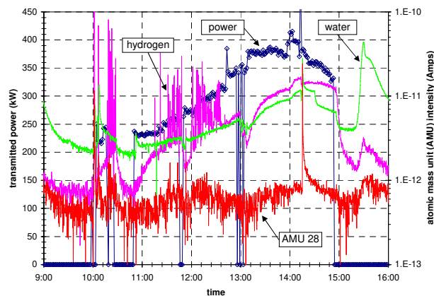
Figure 10: Intensity of residual gases and power level versus time with liquid nitrogen circulating through thermal intercept
