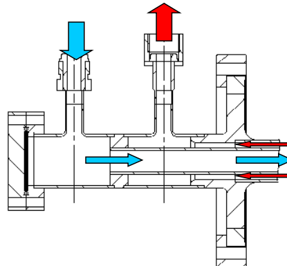
Figure 5: Center conductor coolant inlet and outlet paths
