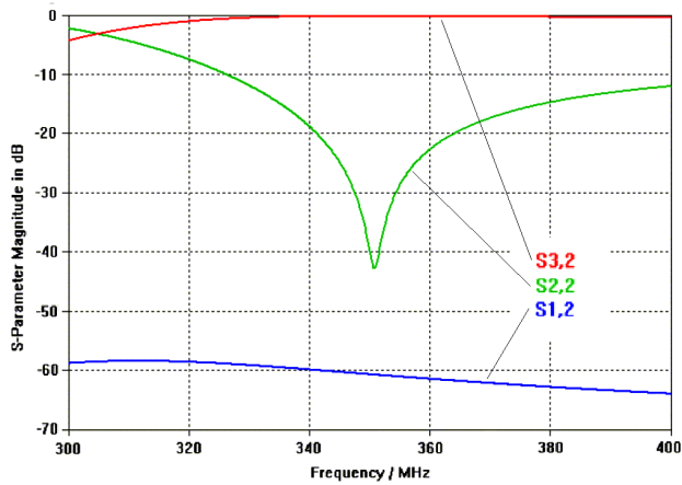
Figure 4: S-parameters for the optimized geometry
