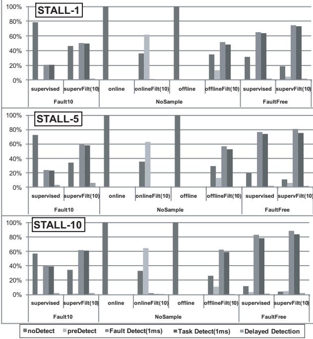
Fig. 4. Average accuracy for STALL
