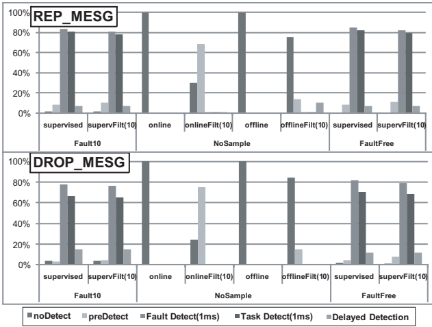
Fig. 5. Average accuracy for DROP_MESG and REP_MESG
