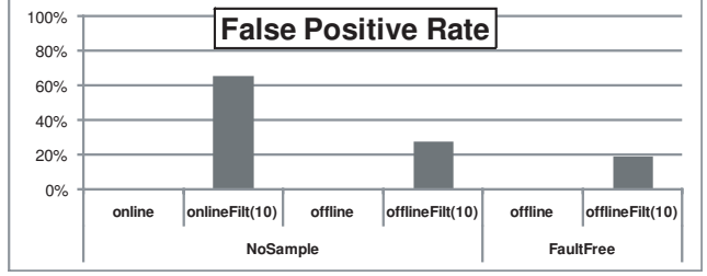
Fig. 6. False Positive Rate on FaultFree set of runs
