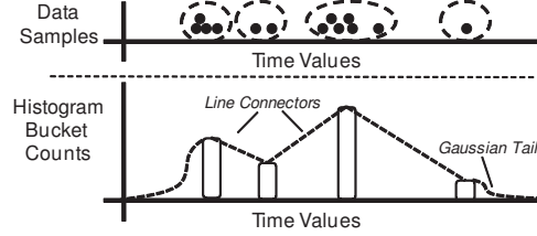
Fig. 1. Example of histogram construction
