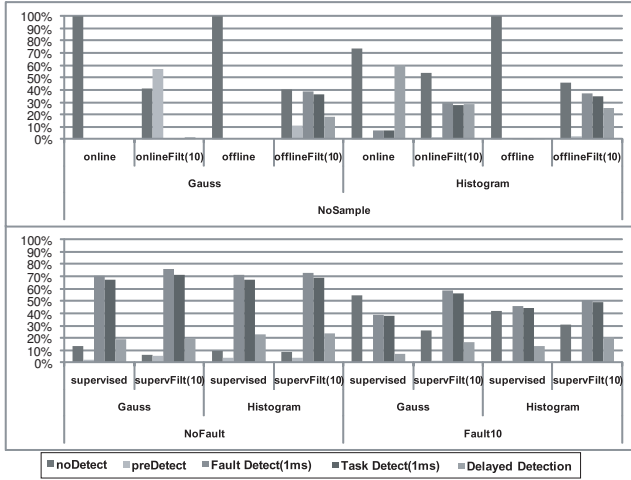
Fig. 2. Average accuracy across all applications and fault types
