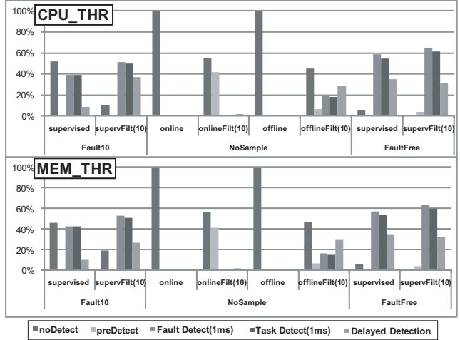
Fig. 3. Average accuracy for CPU_THR and MEM_THR
