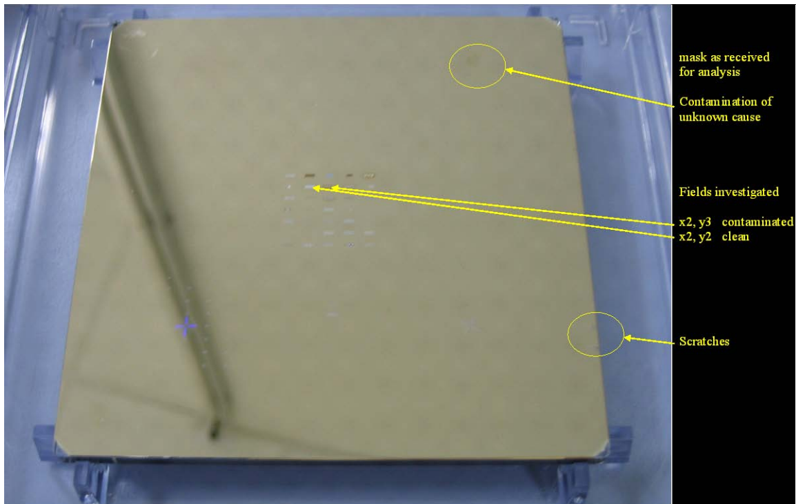
Figure 1: Optical image of the contaminated mask before it was cleaned.
