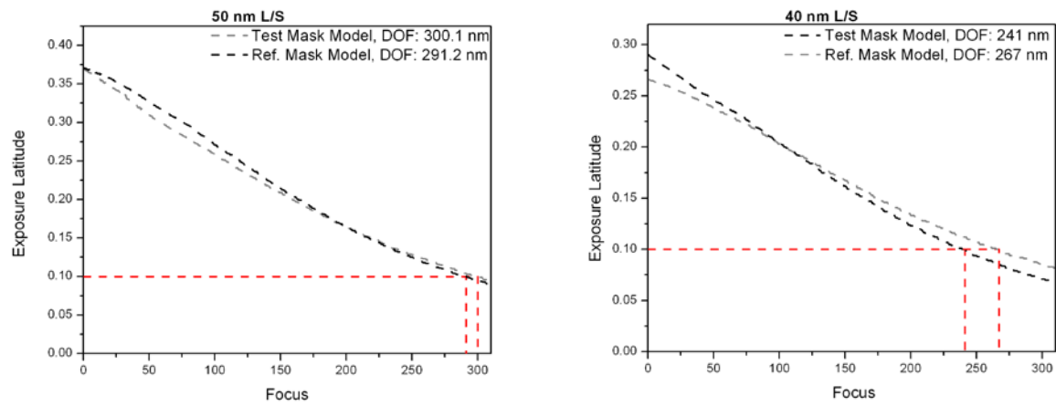
Figure 11: Comparison of exposure latitudes calculated for the E-M Suite modeled aerial images. The modeled data are very closely matched between the two masks.
