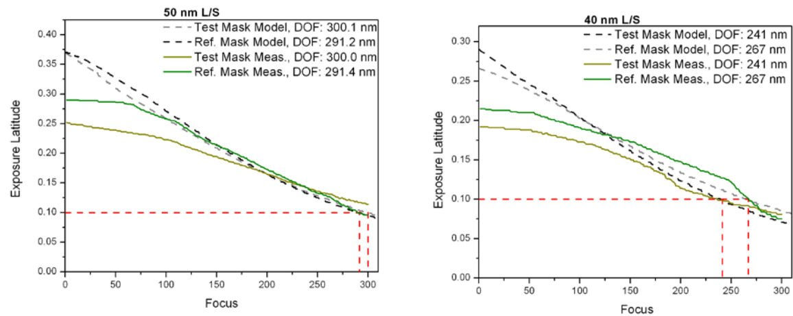
Figure 12: Comparison of exposure latitudes calculated for the MET mask patterned data and for the E-M Suite modeled aerial images.
