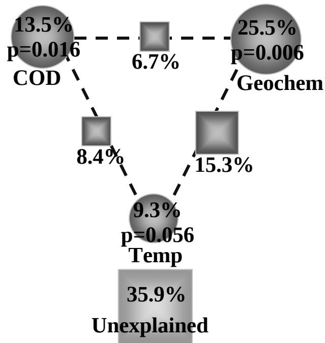
Figure 8. Variance partitioning of environmental variables analyzed by CCA. The diagram represents the relative effects of each variable upon the functional community in FW101-2 and FW102-3. The circles represent the effect of individual variables, by partitioning out the effects of the other variables. The squares between the circles represent the combined effect of the circles on either side of the square. There was no combined effect of all variables. The square at the bottom of each figure represents the effect that could not be explained by any of the variables tested. Variables used in CCA were used for the VPA. COD, chemical oxygen demand; T, temperature; G, geochemical variables (sulfate and uranium). p-values shown were generated during partial CCA.
