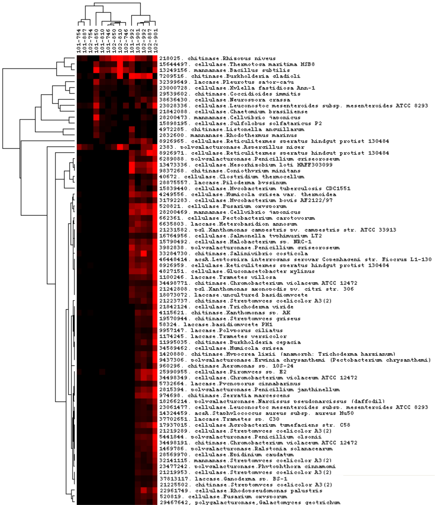
Figure 5. Hierarchical cluster analysis of carbon degradation genes. Genes that were present in at least 4 timepoints were used for cluster analysis. See legend for Fig. 6 for explanation.
