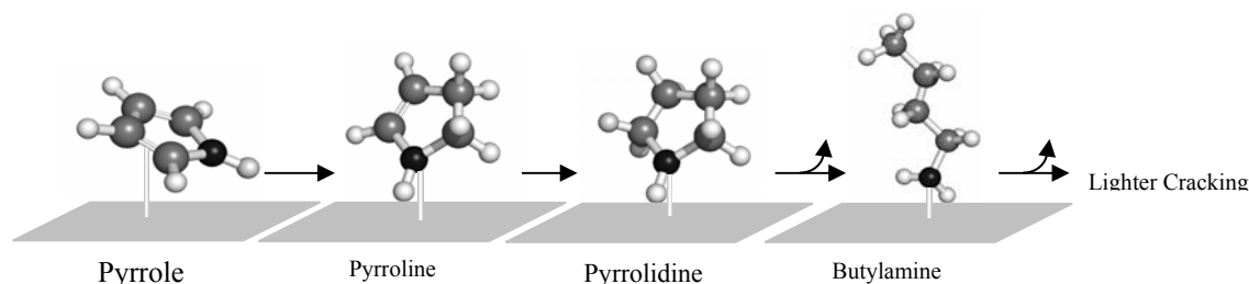
Figure 4.5. Proposed molecular adsorption and reaction pathway over Rh(111). Pyrrole adsorbs in a tilted geometry to the surface bonding through the aromatic \pi system. Once the aromaticity is broken by hydrogenating one of the ring double bonds, the molecule binds to the Rh(111) surface through the lone pair of electrons on nitrogen, which is followed by ring saturation. The molecule may either then desorb to form pyrrolidine, or crack the ring to form butylamine and desorb. On Rh(111) a very small fraction of molecules further decomposes to lighter products.
