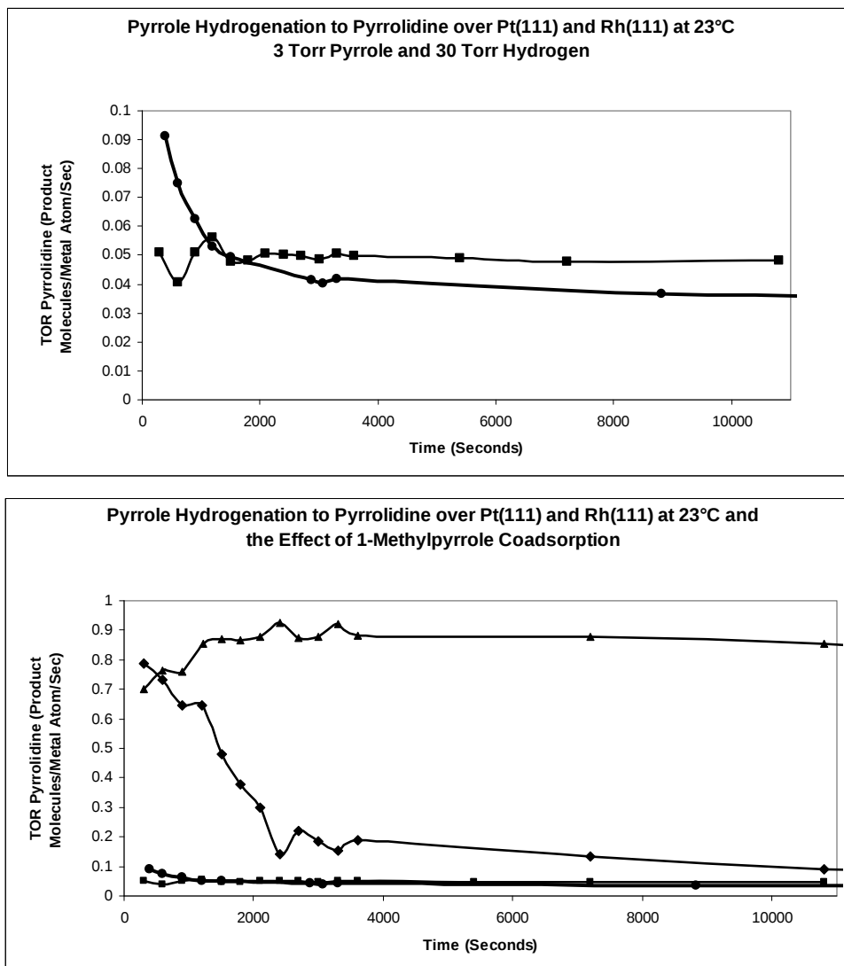
Figure 4.1. Turnover rates (pyrrolidine molecules formed per metal surface atom per second) for the formation of pyrrolidine as a function of time over Pt(111) (—■—) and Rh(111) (—●—) (included in both plots) as compared with Pt(111) dosed with 100 millitorr 1-methylpyrrole prior to reaction (—◆—) and Rh(111) dosed with 100 millitorr 1-methylpyrrole prior to reaction (—▲—) under 3 Torr pyrrole and 30 Torr H 2 .
