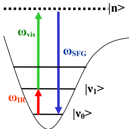
Figure 3.1. Schematic of the infrared-visible SFG-VS process. The term v_0 refers to the vibrational ground state, |v_1\rangle the first vibrational level, and |n\rangle refers to a virtual electronic state.
