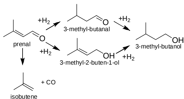
Scheme 7.3. The hydrogenation pathways for prenal.
