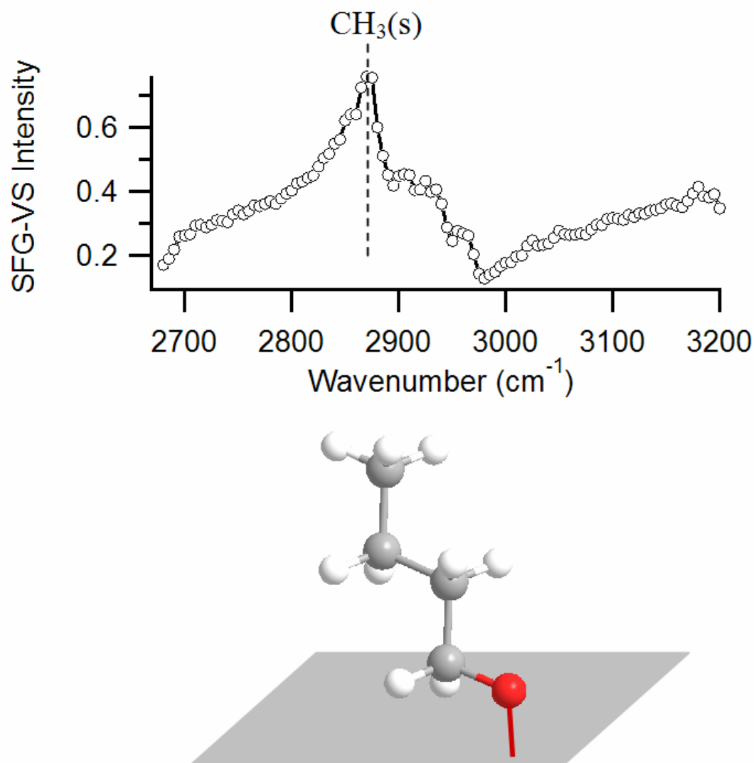
Figure 5.5. SFG-VS reference spectrum of 1 Torr butanol over Pt(111) at 23°C. The dominant \text{CH}_3(\text{s}) peak at 2875\text{ cm}^{-1} indicates that the butanol is standing upright on the surface.
