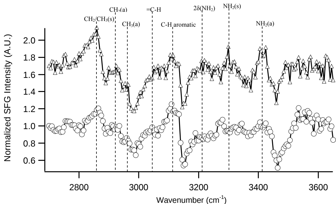
Figure 4.7. SFG vibrational spectra of 3 Torr pyrrole and 30 Torr hydrogen on Pt(111) after exposing the surface to 100 millitorr 1-methylpyrrole for five minutes. The bottom spectrum ( \text{---}\circ\text{---} ) was taken within one hour of reaction time. The top spectrum ( \text{---}\triangle\text{---} ) was taken from one to three hours.
