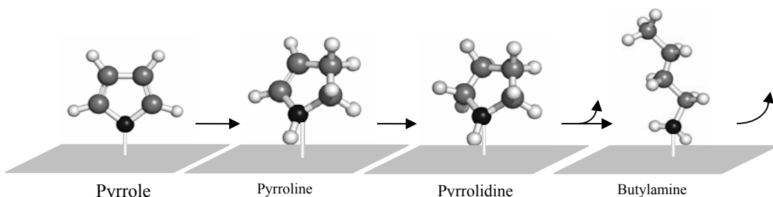
Figure 4.3 Proposed molecular adsorption and reaction pathway over Pt(111). Pyrrole adsorbs perpendicularly by cleaving the N-H bond. Once the aromaticity is broken by the hydrogenation of one of the double bonds, the molecule binds to the Pt(111) surface through the lone pair of electrons on the nitrogen. The subsequent hydrogenation of the ring yields pyrrolidine molecules, some fraction of which may undergo ring-opening and hydrogenation to yield butylamine before desorption.
