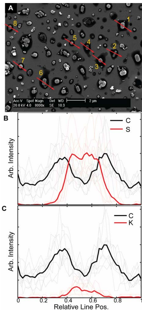
Figure 4. SEM image together with carbon, sulfur and potassium linescans for particles from T0 site. The locations and directions of line scans are shown by the arrows in panel (A). The intensities of characteristic X-rays along the line scans are shown in panels (B) and (C). The line scans confirm that particle cores contain S and K, coated by carbonaceous material. X axis was normalized by the total scan distance. The bold lines represent the X-ray intensities averaged for a number of individual line scans represented by faint lines.
