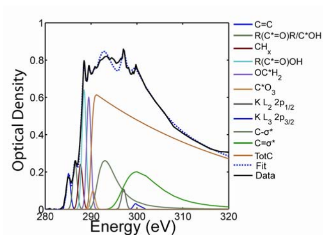
Figure 11. Spectral deconvolution of the averaged C-edge spectrum of particles detected at the T0 site sample. The solid bold black line is the experimental data, the bold blue line is the best fit using the individual peaks labeled in the legend. A list of peak assignments and relative areas for all sites is given in Table 2.
