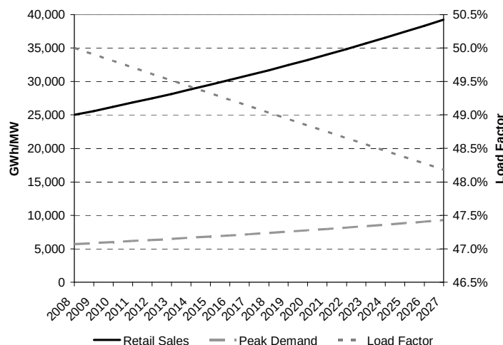
Figure 2. Base Case Forecasted Retail Sales, Peak Demand and Load Factor
