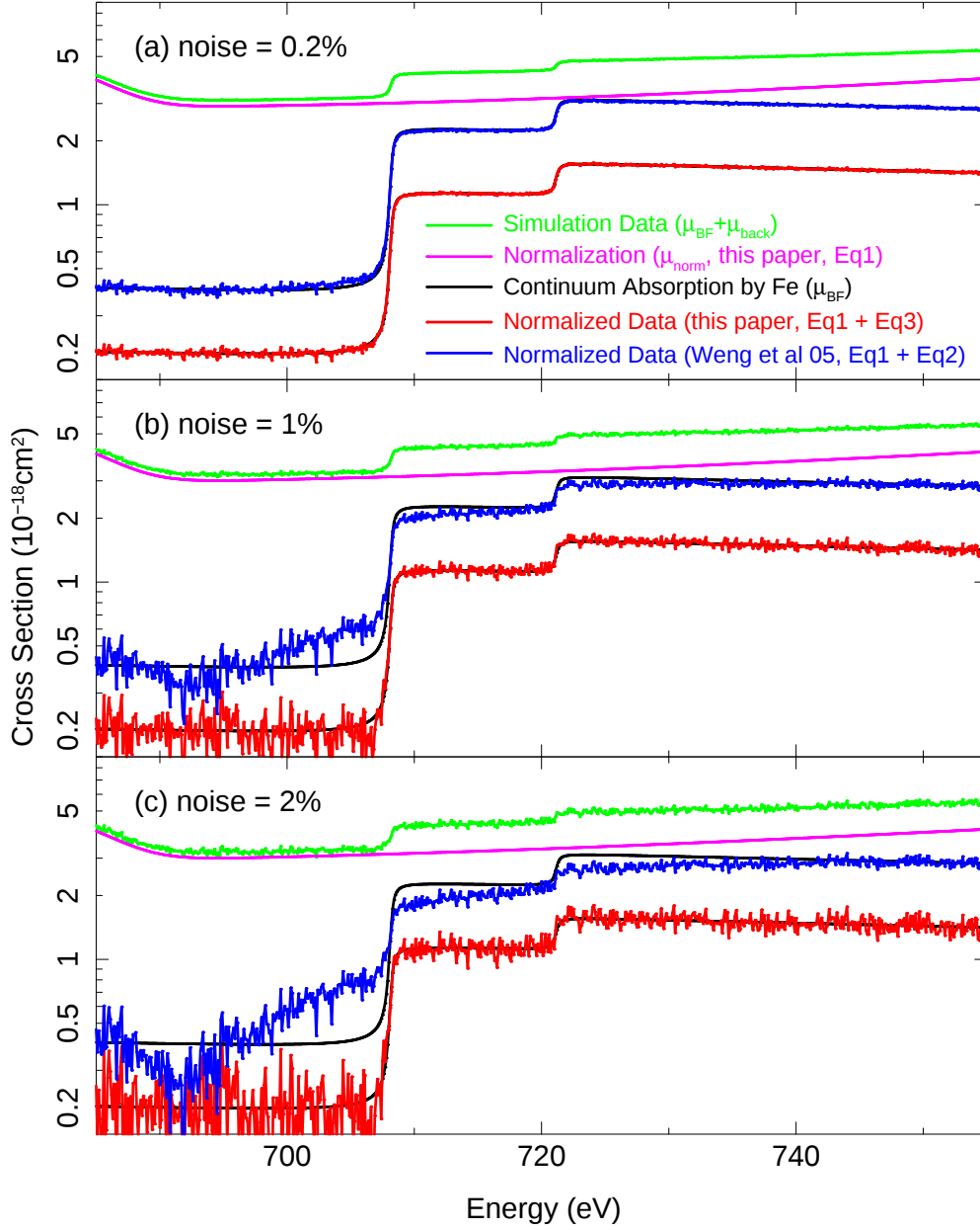
Fig. 3.— A comparison of the normalization technique for compound \gamma -FeOOH, based on Eq. 2 (normalized data based on the method of Weng et al. 2005 shown in blue; arbitrarily scaled up for illustrative purposes), versus its modification (Eq. 3) as proposed in this paper (normalized data shown in red) for simulated data (green) with varying levels of Gaussian distributed noise. The Fe L cross sections of Brennan & Cowen (1992) are shown in black to illustrate goodness of fit. The normalization function of Eq. 1 is show in magenta.
