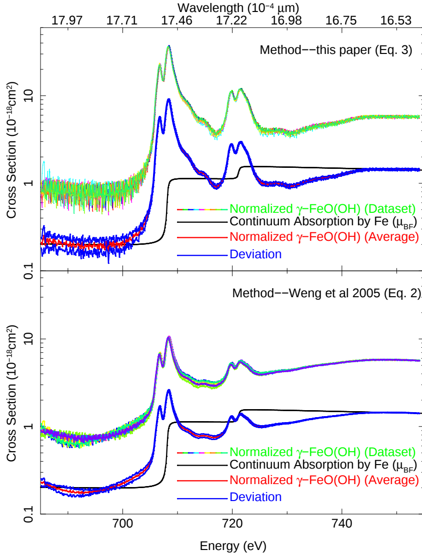
Fig. 4.— A comparison of the cross section normalization technique proposed in this paper (top; Eq. 3) versus that proposed by Weng et al. 2005 (Eq. 2; bottom) for the sample compound \gamma -FeO(OH). In each panel, individual cross section measurements (arbitrarily scaled higher to facilitate plotting purposes) are shown in multicolors, while directly below, the combined normalized data according to the respective methods are shown in red. The blue bracketing this is the standard deviation based on the individual measurements to give sense of measurement differences as a function of energy. The Brennan & Cowen (1992) cross sections are shown in black to compare how the normalization techniques differ.
