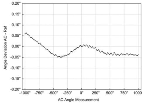
Figure 5: Calibration data (Y-axis of autocollimator) obtained for a SUT (uncoated Zerodur with reflectivity of \sim 4\% ) at a distance of 250 mm from the autocollimator. A circular aperture with a diameter of 15 mm was placed in the front of the SUT and centered on the autocollimator's optical axis.
