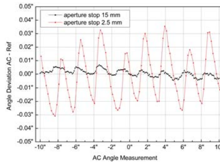
Figure 4: Calibration data (Y-axis of autocollimator) obtained with a sampling of 0.2 arcsec demonstrate periodic deviations in the autocollimator's angular response. The 2.4 arcsec (11.6 \mu rad) period corresponds to the 7 \mu m pixel pitch of the CCD detector. Changing the calibration parameters of the SUT reflectivity (from \sim 100\% to \sim 4\% ) and the aperture diameter [from 2.5 mm (the red line and round dots) to 15 mm (the black line and square dots)] results in reducing the periodic deviations by a factor of >10 .
