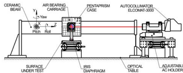
31 32 Figure 1: Simplified model of an autocollimator-based profiler. 33
