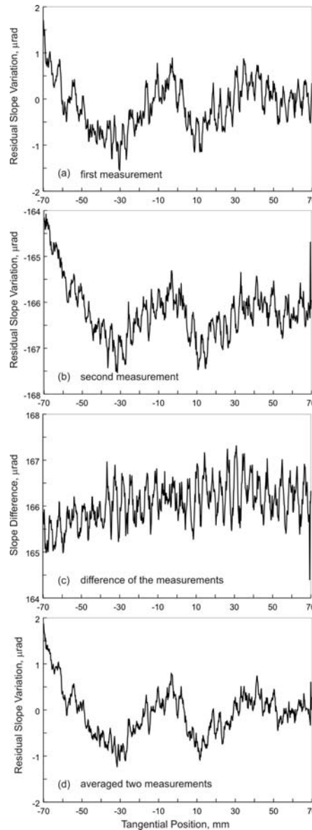
Figure 10: DLTP measurements of the 15 m spherical test mirror. (a) The residual slope trace measured in the first run of {F-R-R-F-R-F-F-R} scans. The best-fit spherical shape with a radius of curvature of 14.977 m is subtracted. (b) DLTP measurement similar to that of (a) but with the mirror tilted in the tangential direction by 144 \mu\text{rad} . (c) Difference of the measurements shown in plots (a) and (b). This slope trace can be thought of as twice the self calibration function of the instrument. (d) Residual slope variation trace averaged over the measurements presented in plots (a) and (b). The systematic oscillation is significantly suppressed and the resulting trace is a more reliable measure for the surface slope variation.
