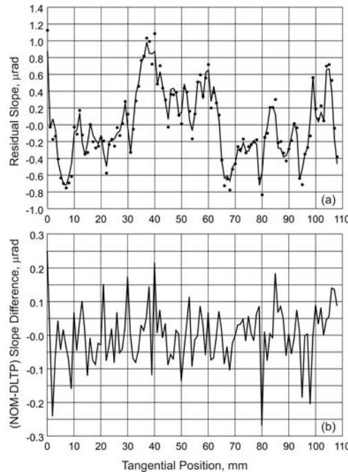
Figure 12: (a) The residual slope variation of the S3 reference mirror measured with the DLTP (solid line) and NOM (solid dots). The best-fit spherical surface shape with a radius of curvature of 1287.5 m (DLTP data) and 1280.4 (NOM data) was subtracted. (b) Difference of the measurements in (a).
