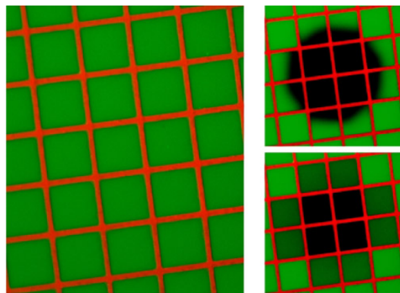
Figure 2: A supported lipid bilayer (green) patterned by a grid of microcontact printed bovine serum albumin (red, corral size 50 x 50 \mu m), one of the many materials that can be used to create membrane corrals. A photobleached spot (black, upper right panel) relaxes (20 minutes later; lower right panel) demonstrating lateral fluidity, confinement and complete mixing within the corralled regions [35].
